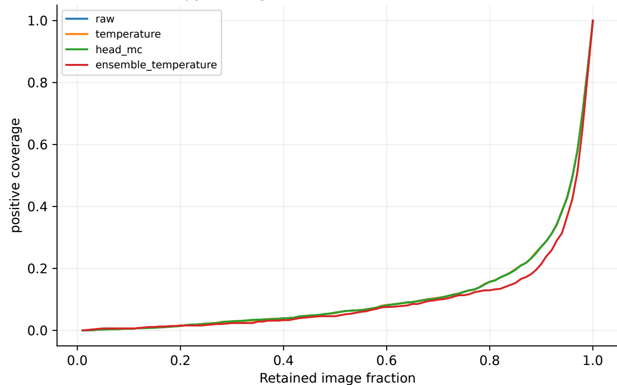
densenet121: pleural effusion - vinbig Entropy ranking; source-frozen decision threshold
