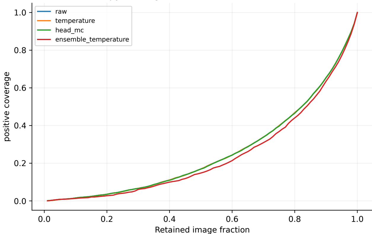
resnet18: cardiomegaly - chexpert Entropy ranking; source-frozen decision threshold
