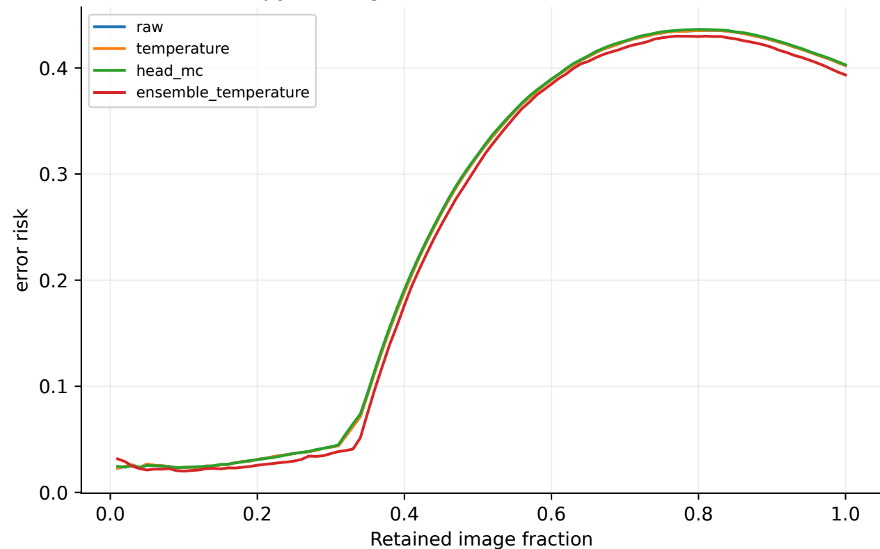
resnet18: pleural effusion - chexpert Entropy ranking; source-frozen decision threshold
