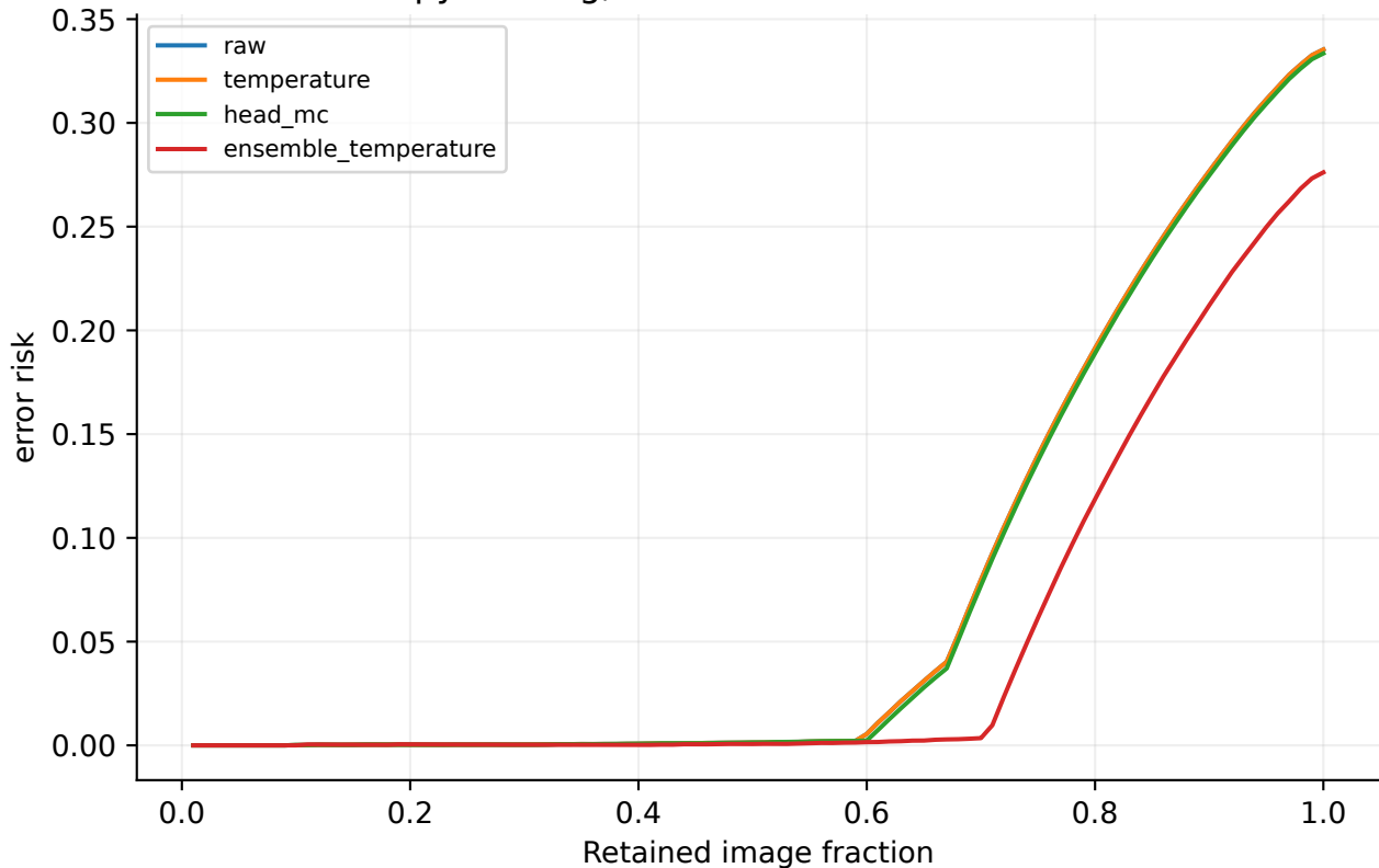
resnet18: cardiomegaly - nih Entropy ranking; source-frozen decision threshold
