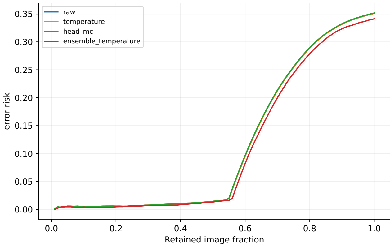
resnet18: pleural effusion - nih Entropy ranking; source-frozen decision threshold
