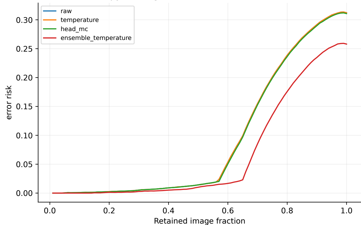
resnet18: cardiomegaly - vinbig Entropy ranking; source-frozen decision threshold
