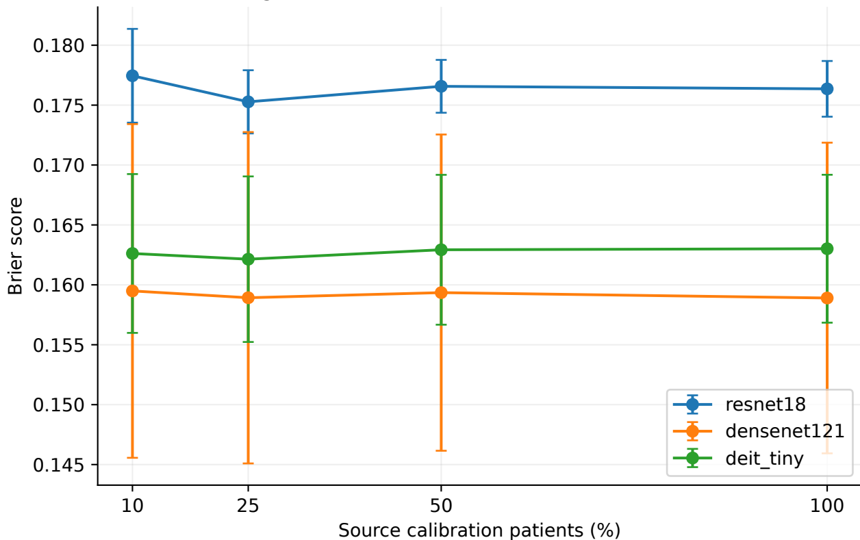
Calibration-label budget: pleural effusion - chexpert Full training data; failed low-event fits omitted and tabulated
