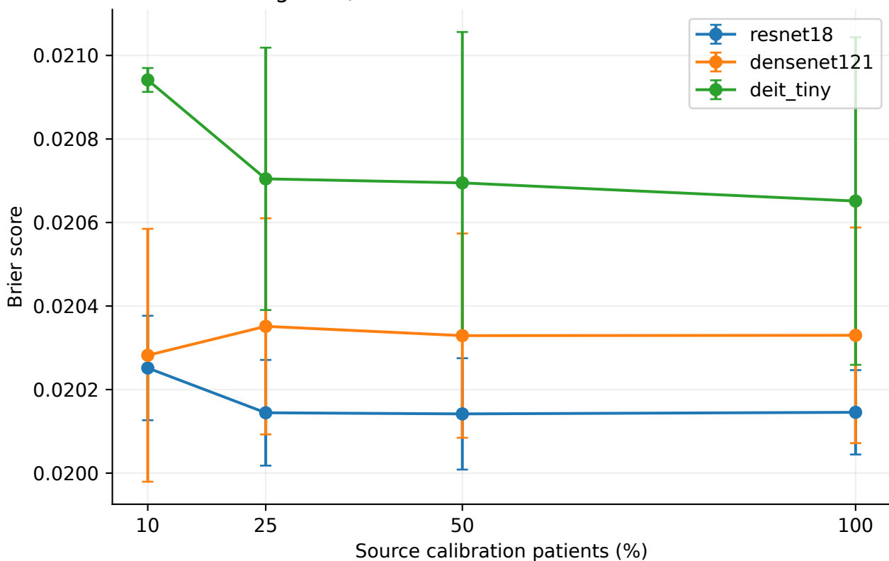
Calibration-label budget: cardiomegaly - nih Full training data; failed low-event fits omitted and tabulated
