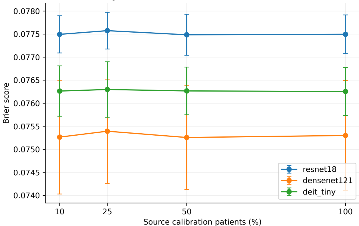
Calibration-label budget: pleural effusion - nih Full training data; failed low-event fits omitted and tabulated
