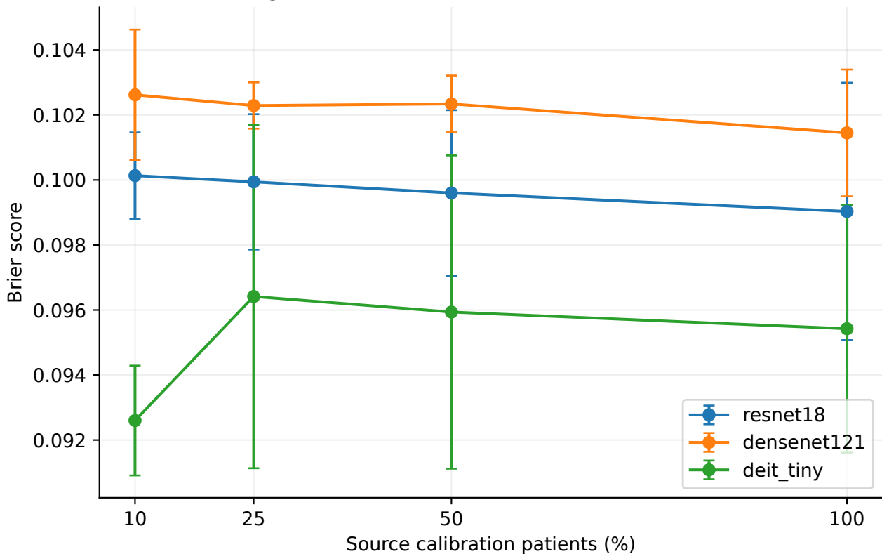
Calibration-label budget: cardiomegaly - vinbig Full training data; failed low-event fits omitted and tabulated
