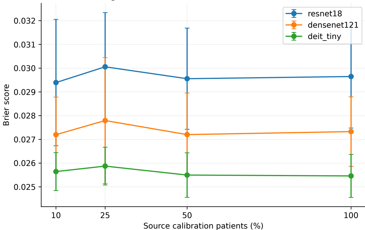
Calibration-label budget: pleural effusion - vinbig Full training data; failed low-event fits omitted and tabulated
