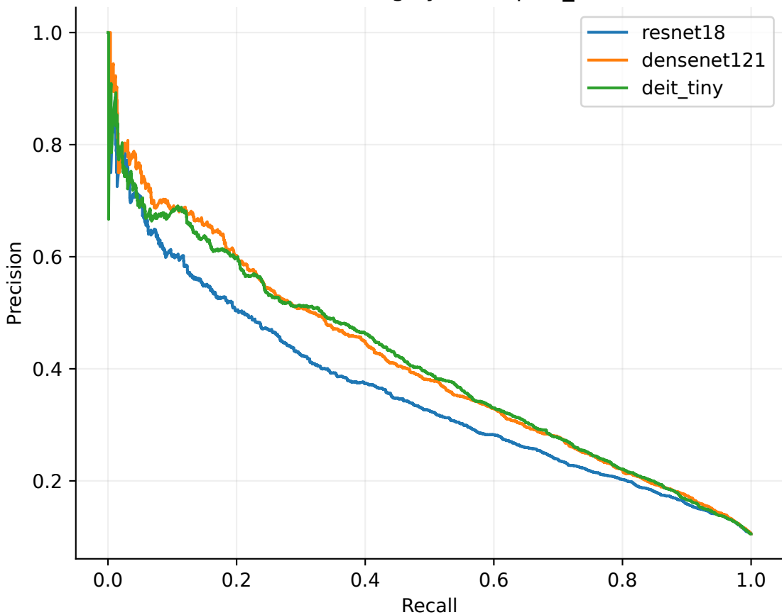
PR: cardiomegaly - chexpert_test
