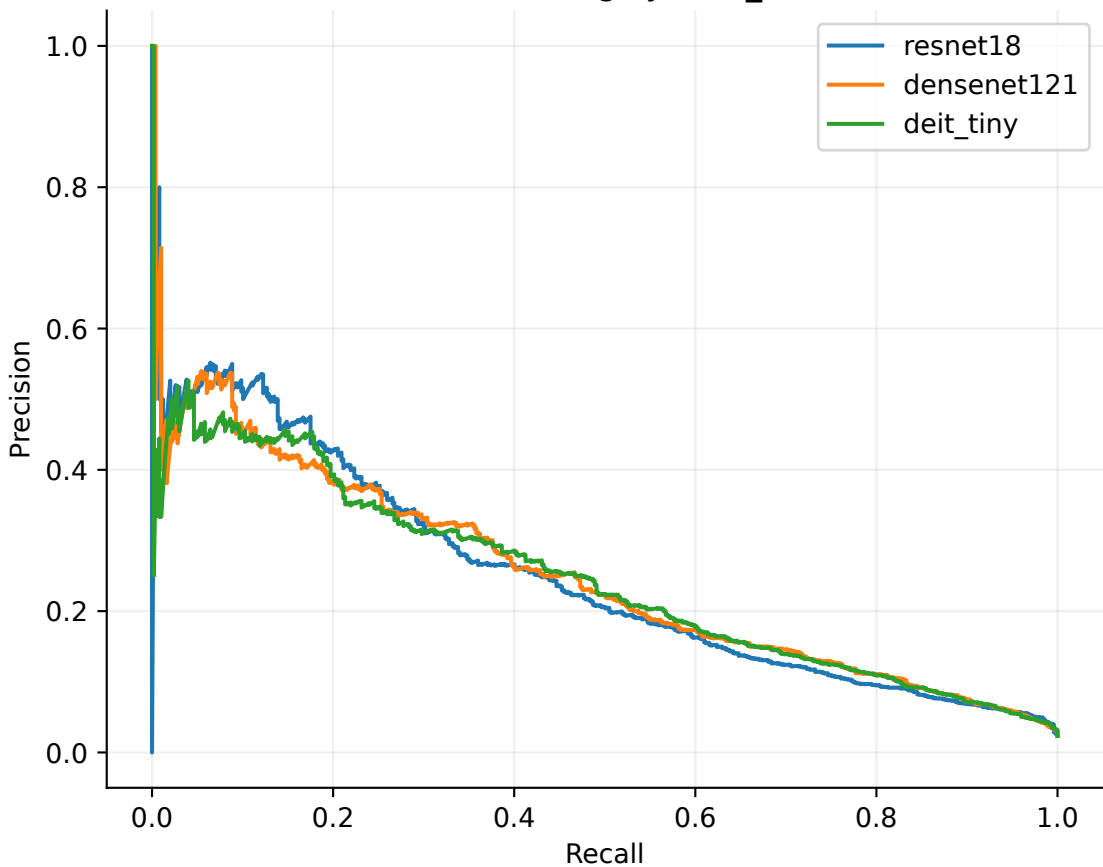
PR: cardiomegaly - nih_test
