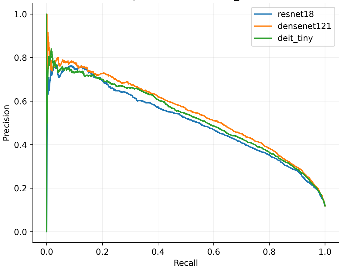
PR: pleural effusion - nih_test
