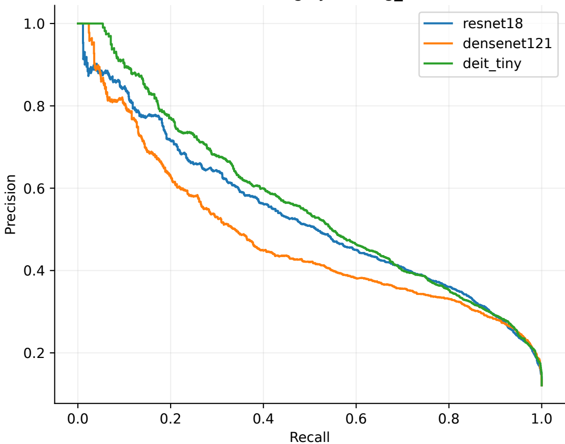
PR: cardiomegaly - vinbig_test
