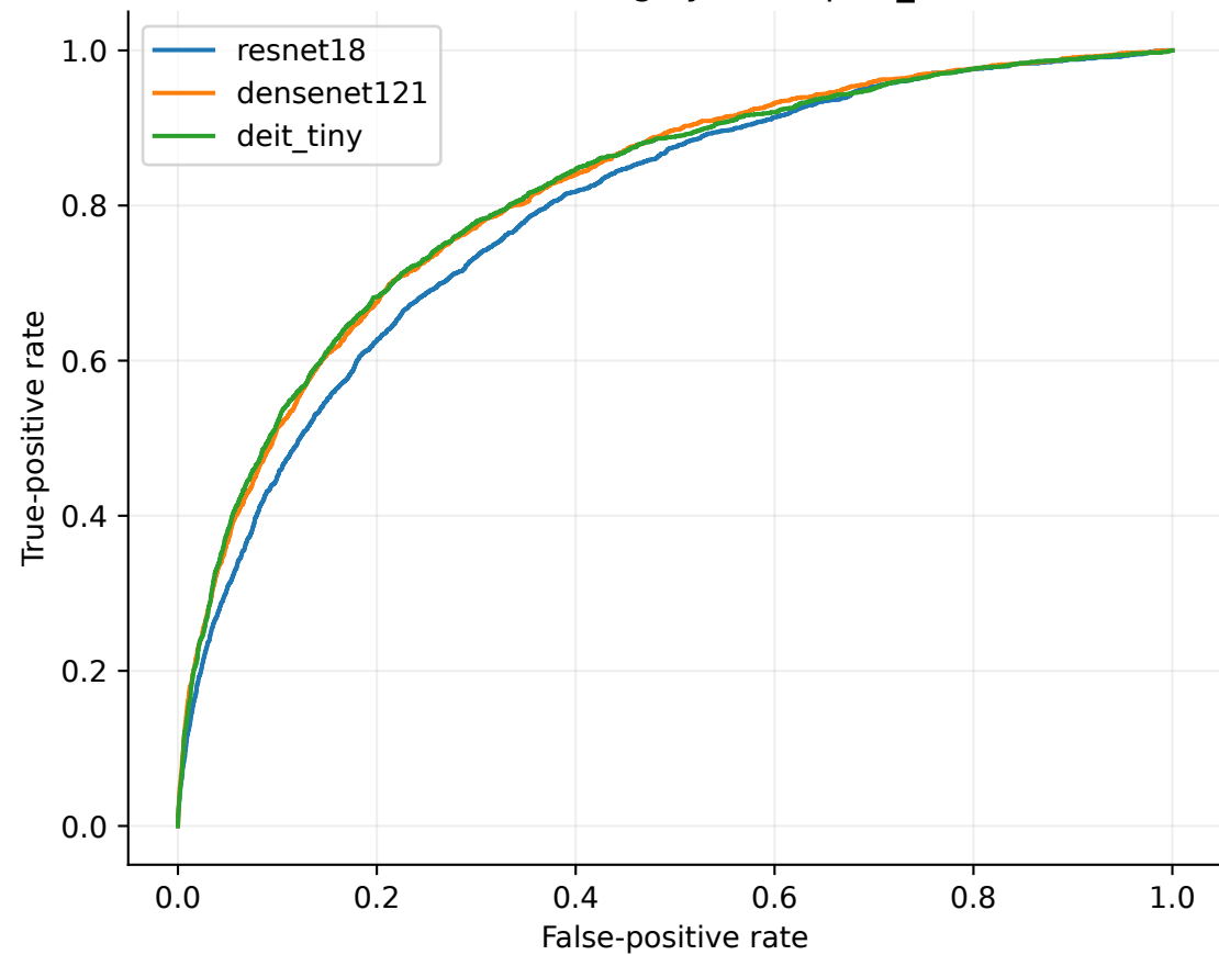
ROC: cardiomegaly - chexpert_test
