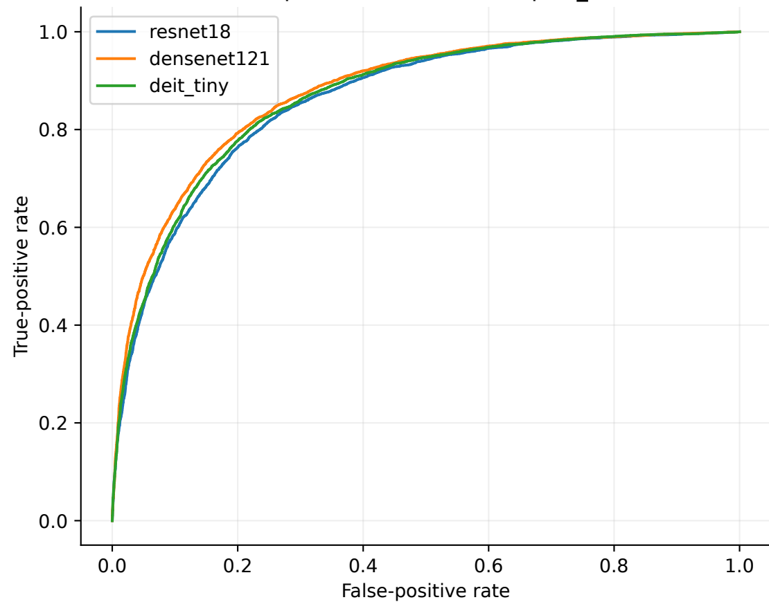
ROC: pleural effusion - chexpert_test
