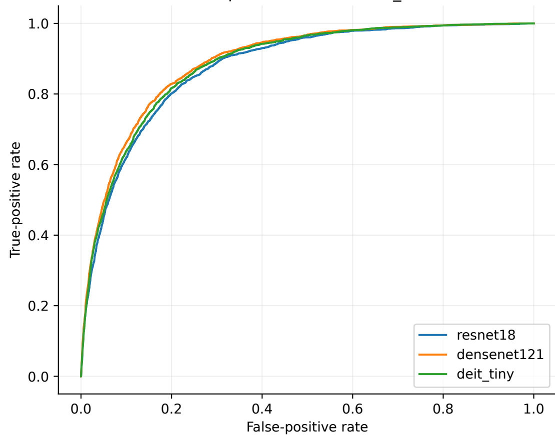
ROC: pleural effusion - nih_test
