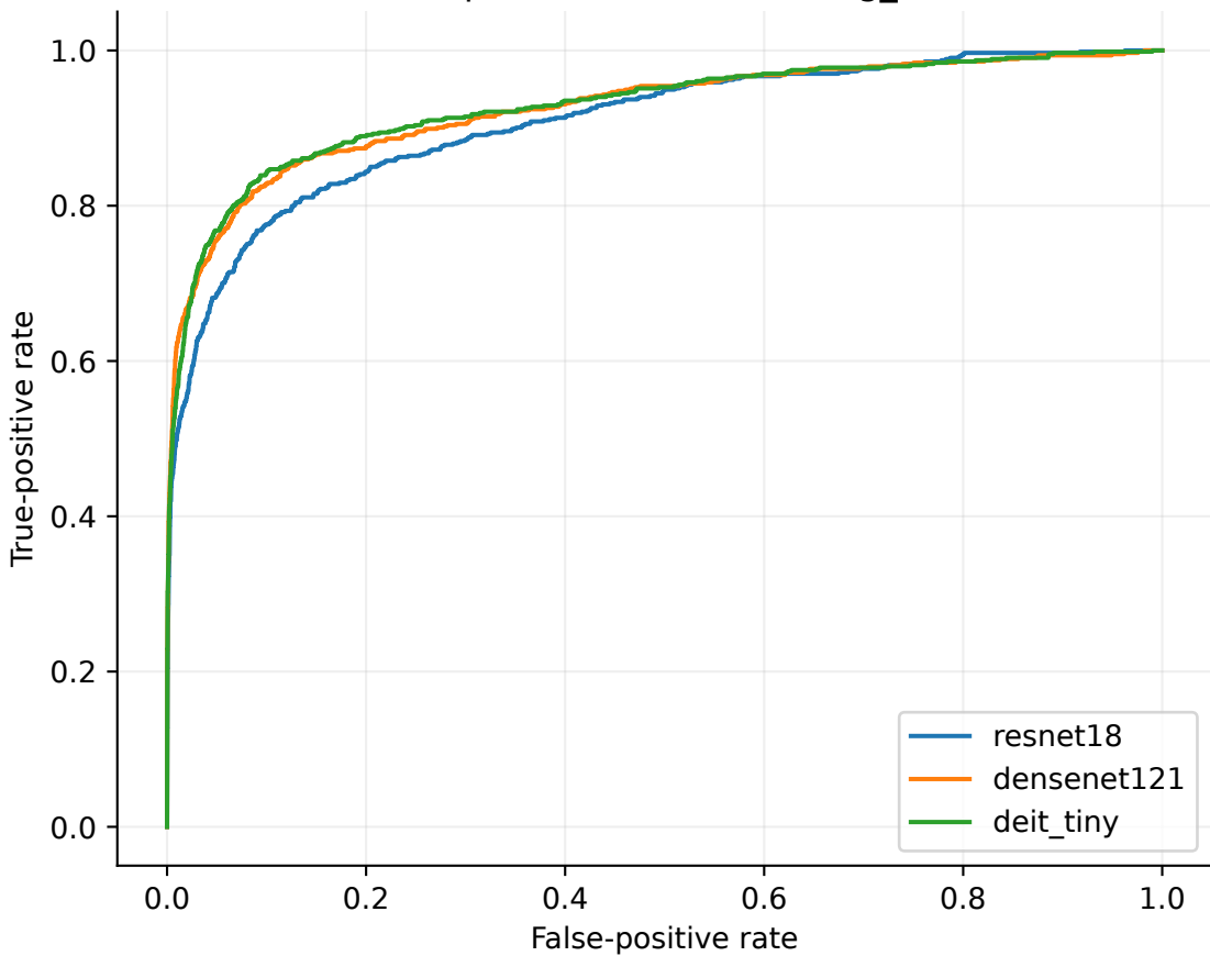
ROC: pleural effusion - vinbig_test
