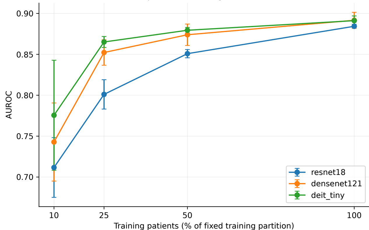
Cardiomegaly - nih Source temperature scaling; mean \pm seed SD
