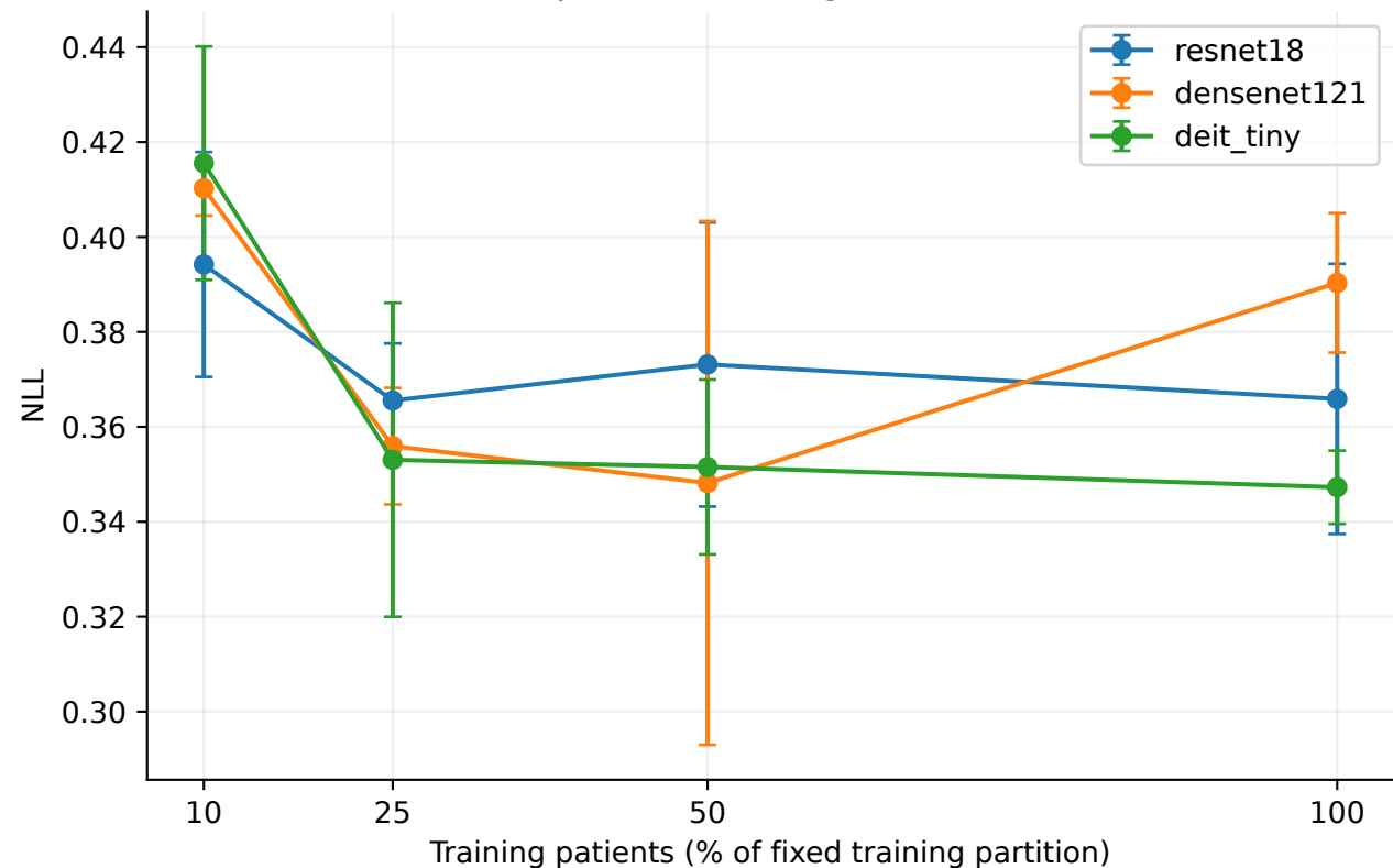
Cardiomegaly - vinbig Source temperature scaling; mean \pm seed SD
