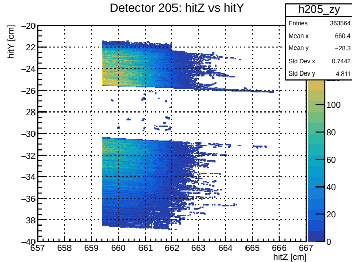
Detector 205: hitZ vs hitY
