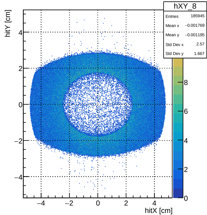
hitX vs hitY - Detector 8: Quad 4 Exit
