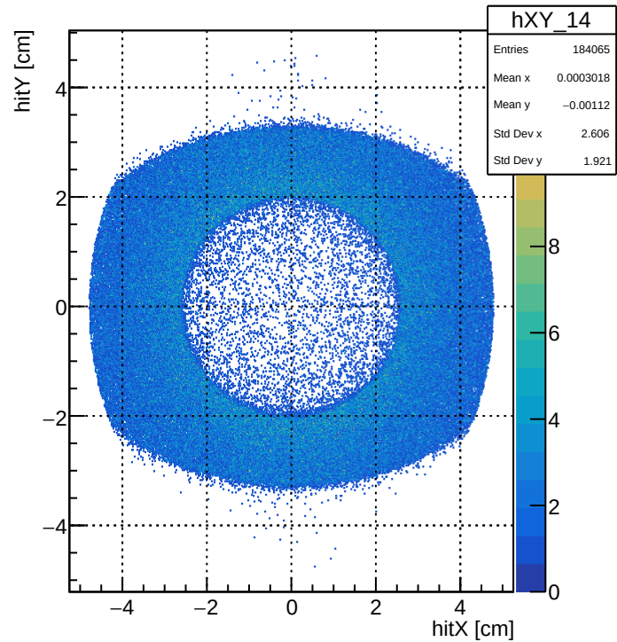
hitX vs hitY - Detector 14: Dipole Entrance
