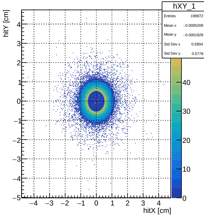
hitX vs hitY - Detector 1: Quad 1 Entrance
