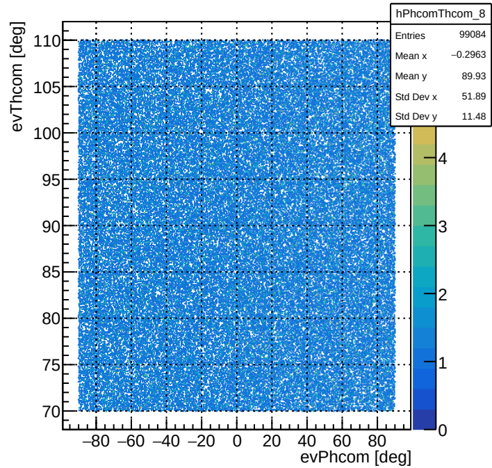
evPhcom vs evThcom - Detector 8: Quad 4 Exit
