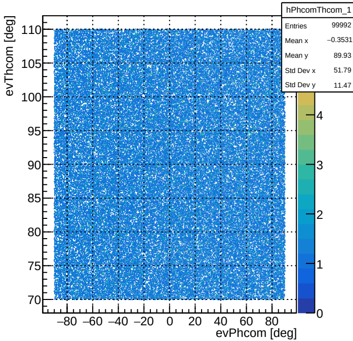
evPhcom vs evThcom - Detector 1: Quad 1 Entrance
