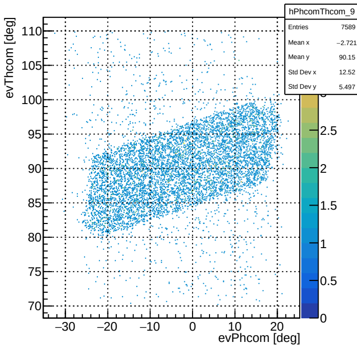
evPhcom vs evThcom - Detector 9: Moller Detector
