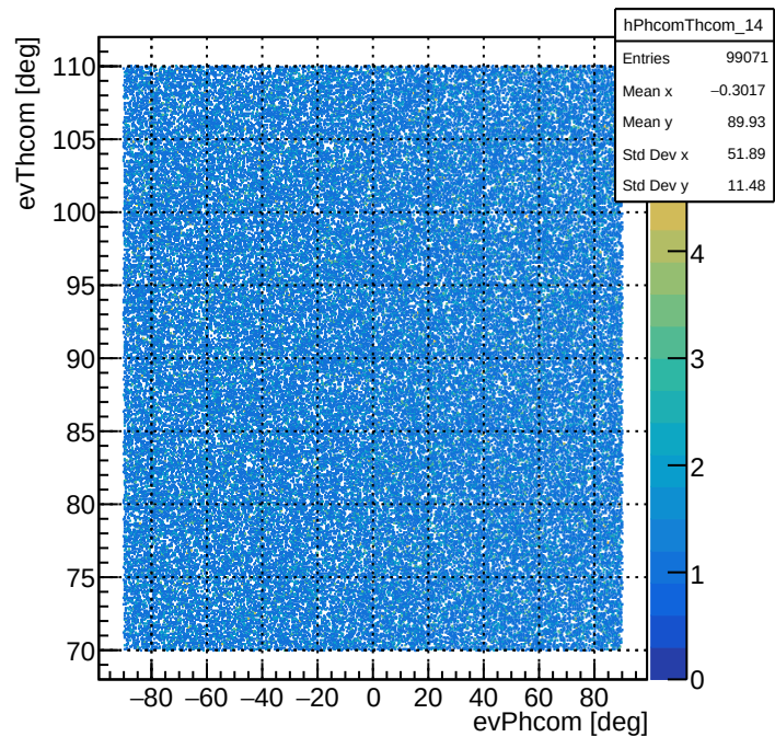
evPhcom vs evThcom - Detector 14: Dipole Entrance
