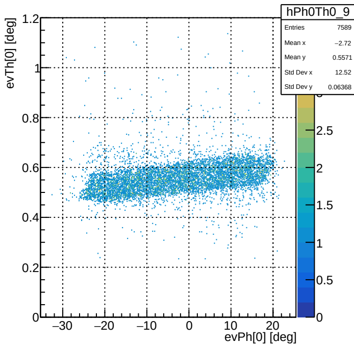
evPh[0] vs evTh[0] (degrees) - Detector 9: Moller Detector
