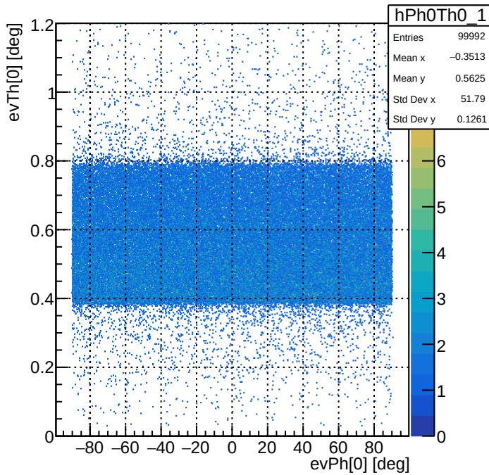
evPh[0] vs evTh[0] (degrees) - Detector 1: Quad 1 Entrance
