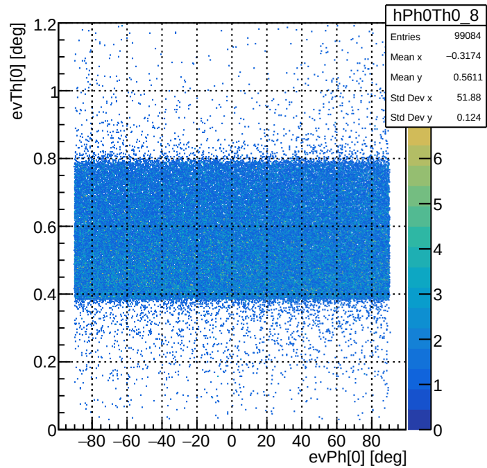
evPh[0] vs evTh[0] (degrees) - Detector 8: Quad 4 Exit
