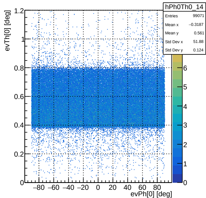
evPh[0] vs evTh[0] (degrees) - Detector 14: Dipole Entrance
