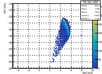
Mask of Kryptonite (Mask Interacts) Det202
