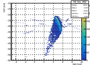
Mask of Tungsten (Mask Interacts) Det202
