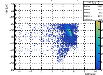
Mask of Carbon (Mask Interacts) Det9
