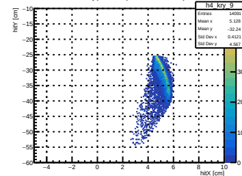
Mask of Kryptonite (Mask Interacts) Det9
