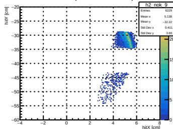
Mask of Carbon (Mask Doesn't Interact) Det9
