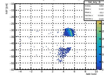
Mask of Tungsten (Mask Interacts) Det9
