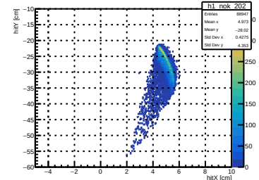
Mask of Tungsten (Mask Doesn't Interact) Det202
