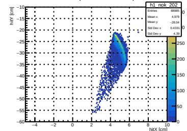
Mask of Carbon (Mask Doesn't Interact) Det202
