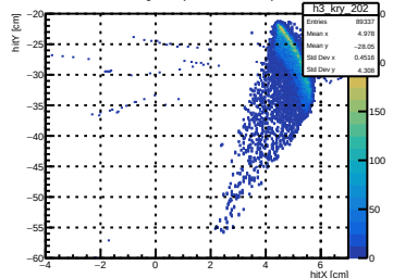
Mask of Tungsten (Mask Interacts) Det202
