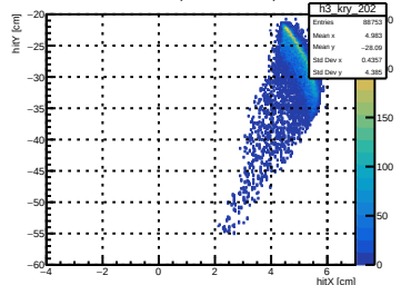
Mask of Carbon (Mask Interacts) Det202
