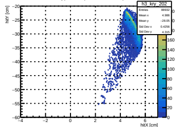
Mask of Kryptonite (Mask Interacts) Det202
