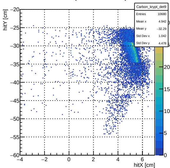
Carbon (Mask Interacts)
