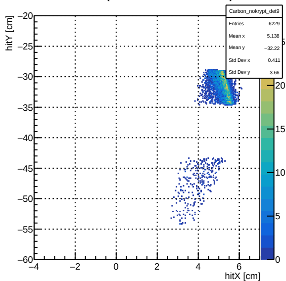
Carbon (Mask Doesn't Interact)
