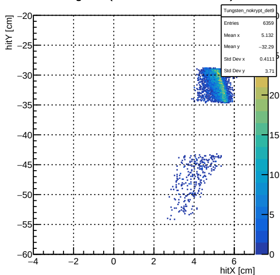
Tungsten (Mask Doesn't Interact)
