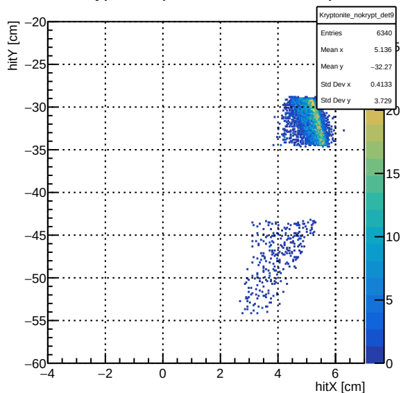
Kryptonite (Mask Doesn't Interact)
