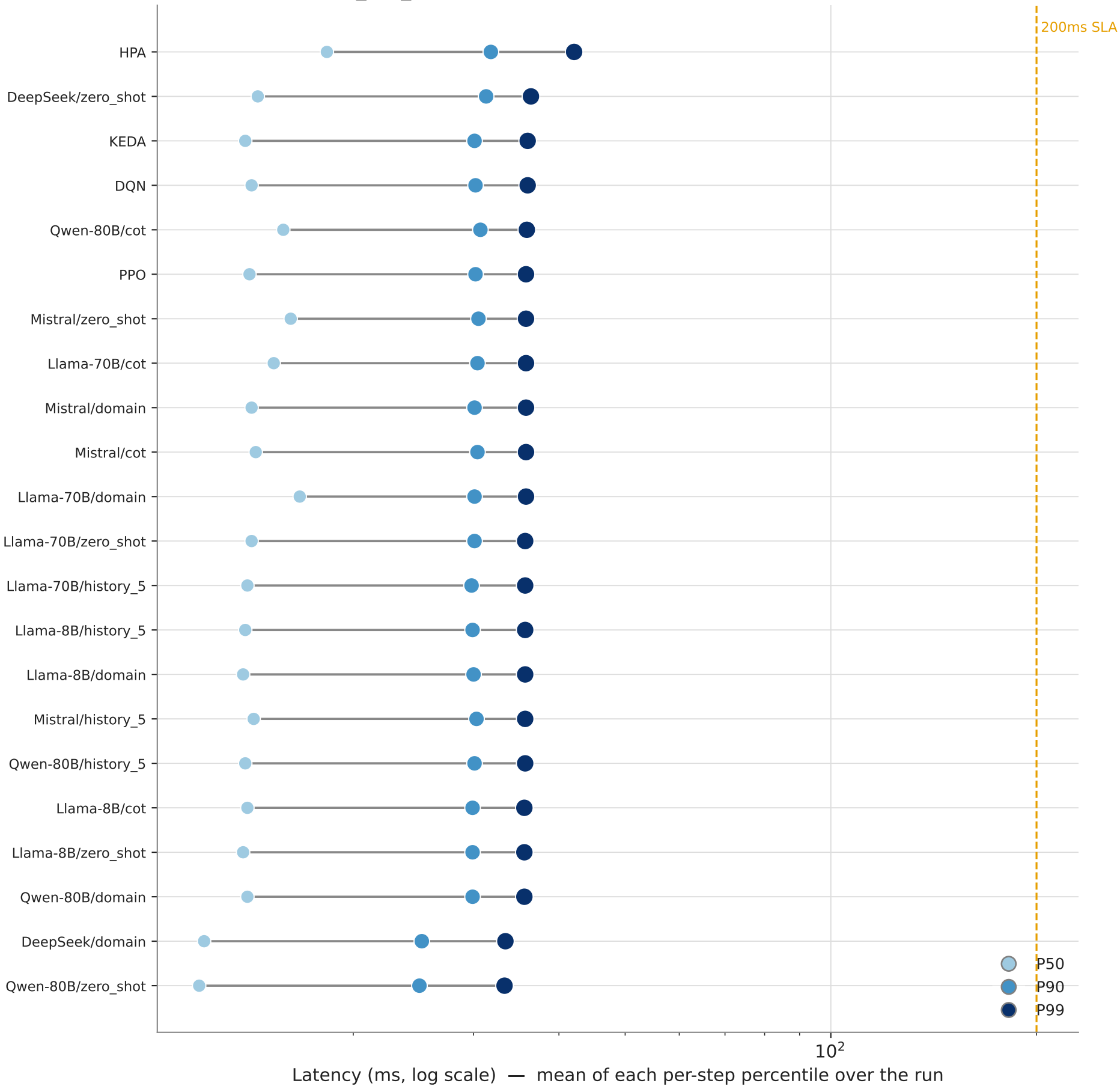
Real cluster (results_k8s_v2, io workload): P50 → P90 → P99 latency spread per config
