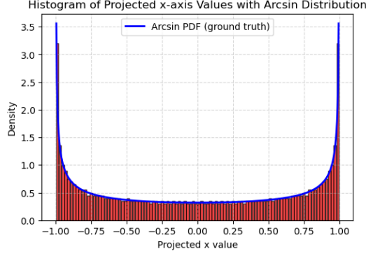
Figure 1: Distribution of roots of Chebyshev polynomials projected onto the x-axis (arcsine distribution // TODO: FIX FORMATTING ).
