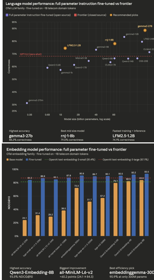
Figure 1: OTel fine-tuning improves language-model correctness and embedding retrieval quality; larger LLMs generally raise the correctness upper envelope.
