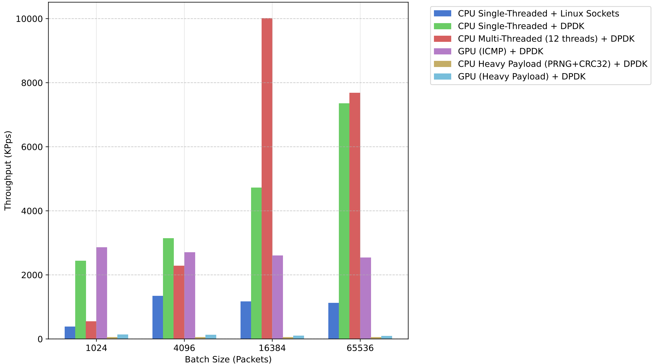
End-to-End Pipeline Comparison: Kernel vs. Kernel-Bypass (DPDK)
