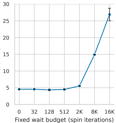
Base backup elapsed time (s)
