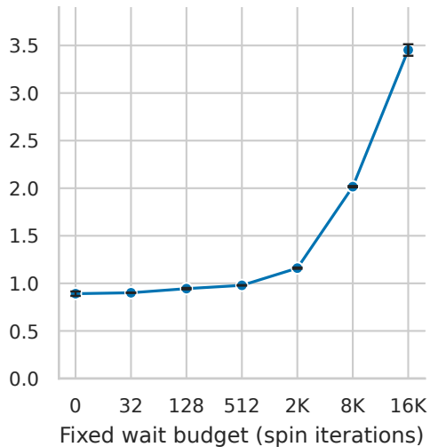
Transaction p99 latency (ms)
