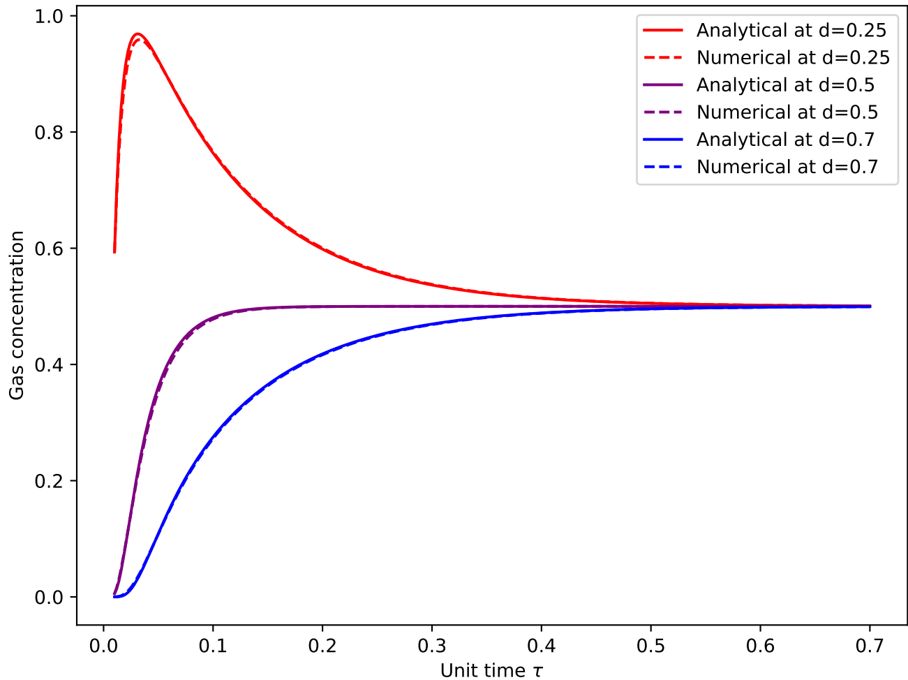
Concentration variation over time, at fixed distances
