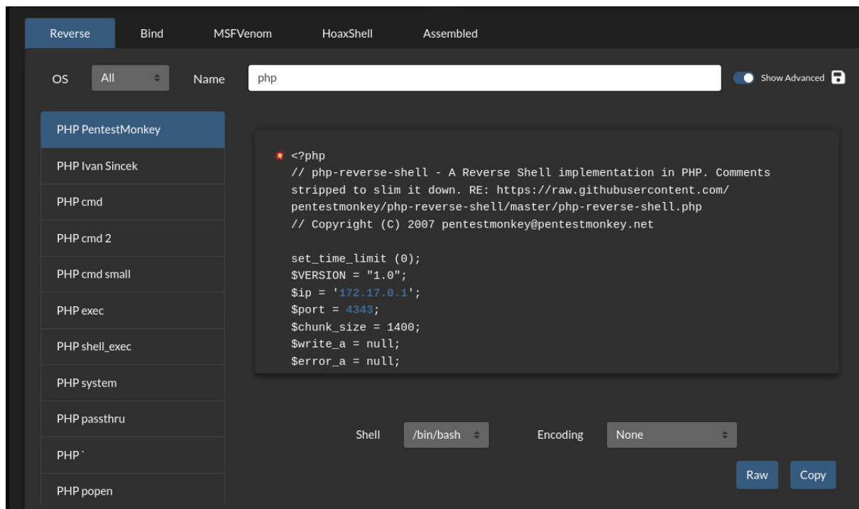
Figure 7: Reverse Shell
