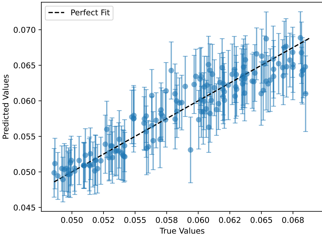
Prediction vs. True with Uncertainty (Laplace)
