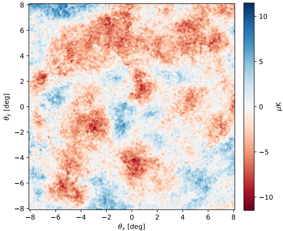
Original kSZ Map (True \tau = 0.0487 )
