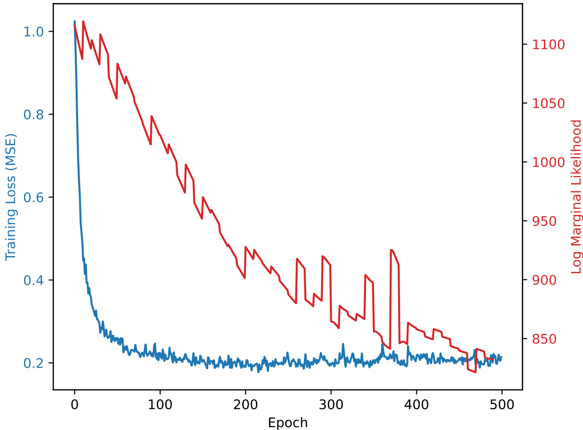
Training Loss vs. Marginal Likelihood
