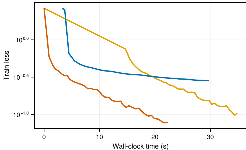
(b) Train loss vs. time
