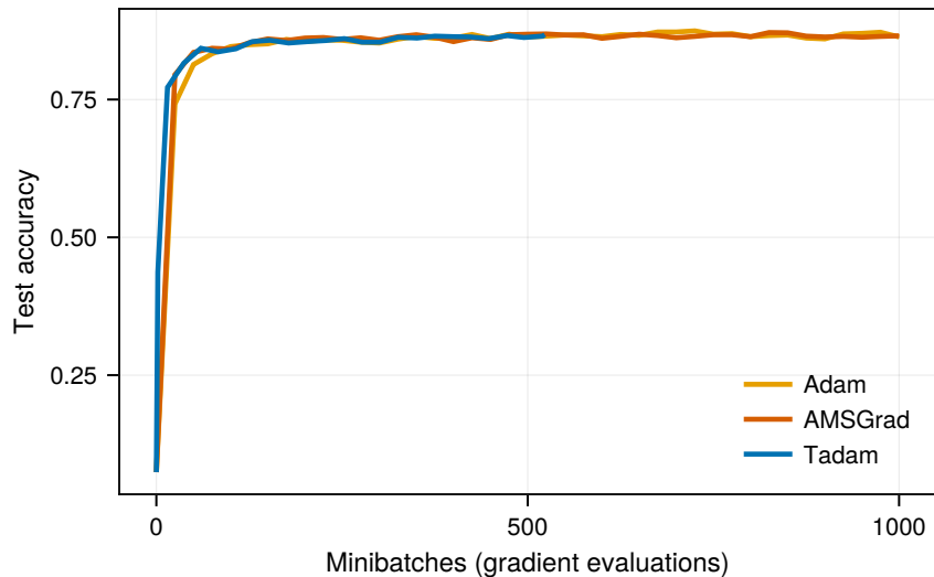
(c) Test accuracy vs. gradient evaluations
