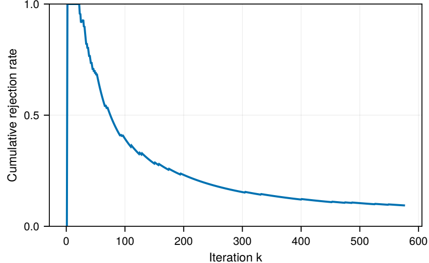
(f) TR step rejection rate over training (Tadam)
