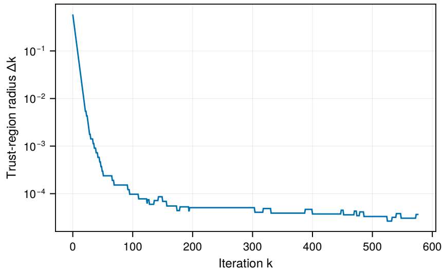
(e) Adaptive step size: \Delta k over iterations (Tadam)
