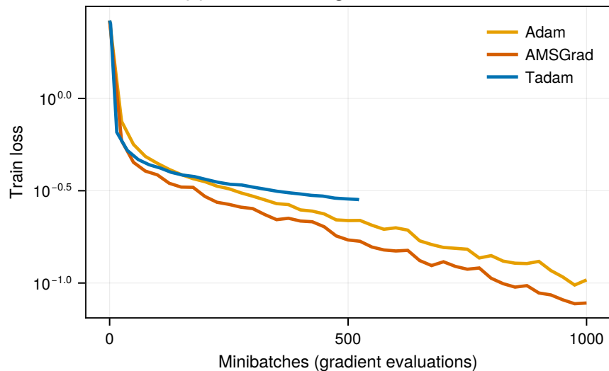
(a) Train loss vs. gradient evaluations
