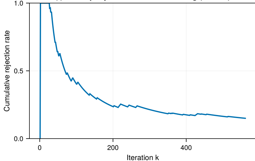
(f) TR step rejection rate over training (Tadam)
