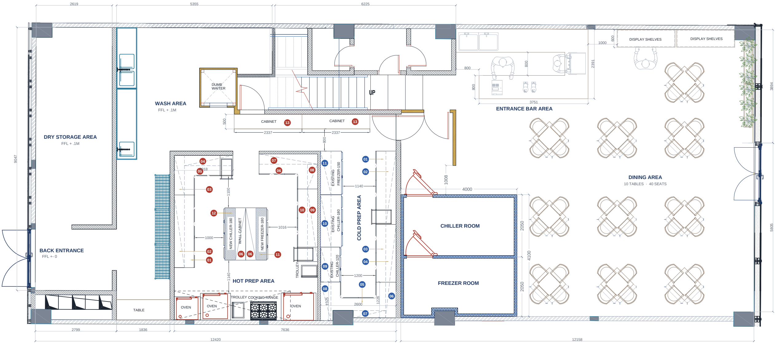
01 GROUND FLOOR LAYOUT A-01 KITCHEN EQUIPMENT & DINING ARRANGEMENT | SCALE 1:80 @ A3
