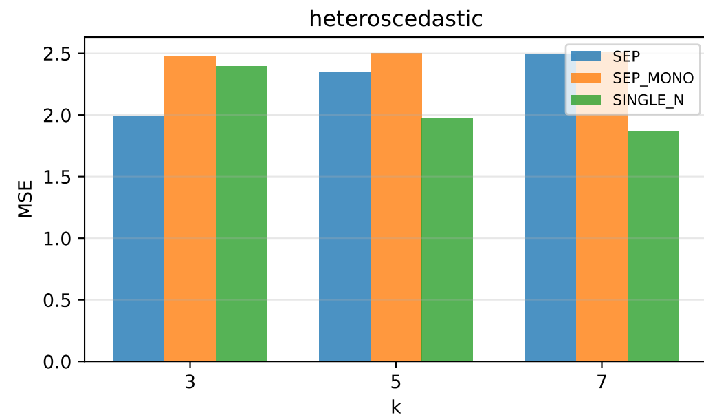
MSE by variant — D1 (strategy) and D3 (monotonic constraints)
