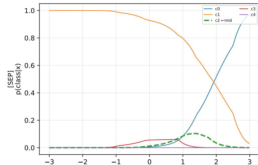
exponential k=5 | mid_idx=2
