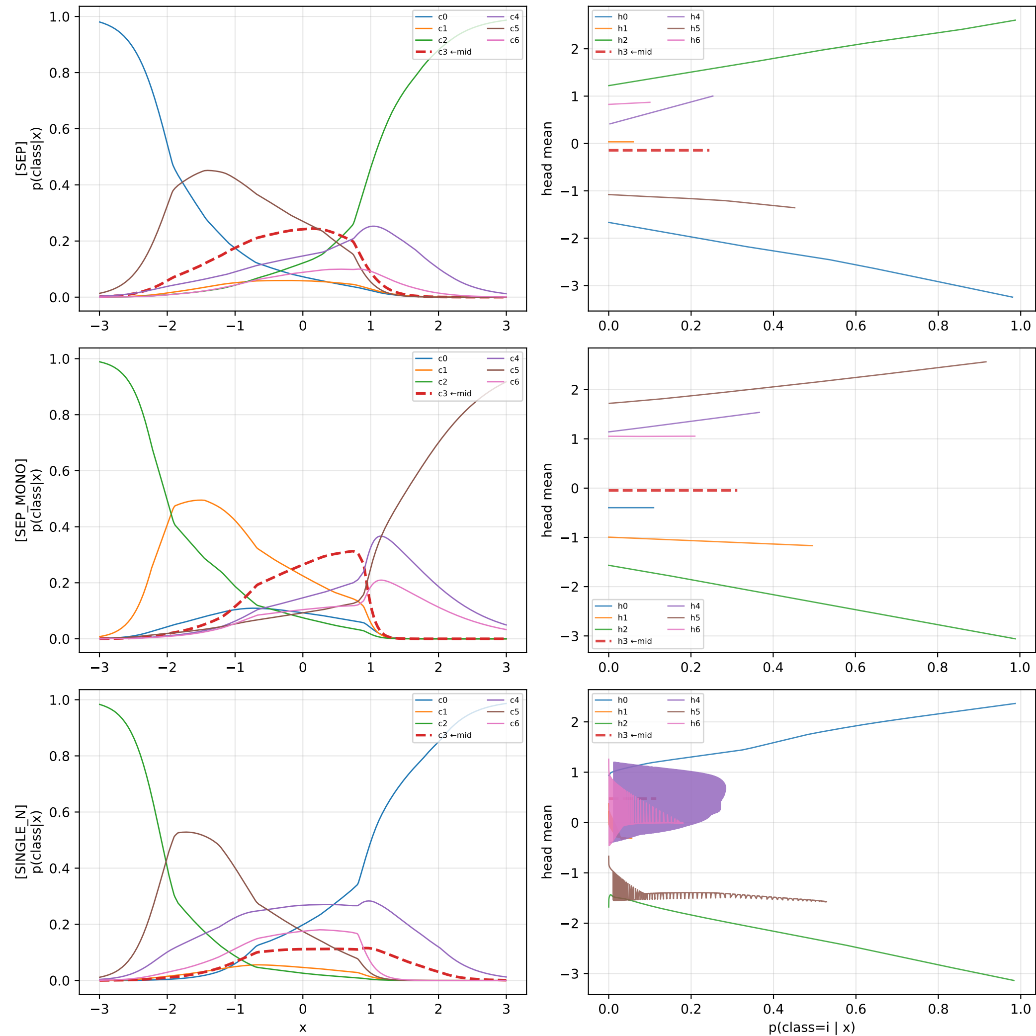
bimodal k=7 | mid_idx=3
