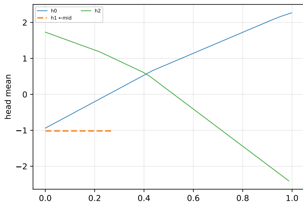
piecewise k=3 | mid_idx=1
