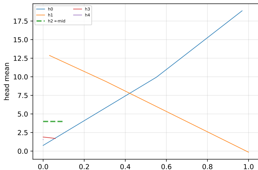
exponential k=5 | mid_idx=2
