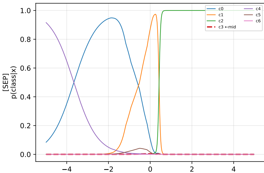
heteroscedastic k=7 | mid_idx=3
