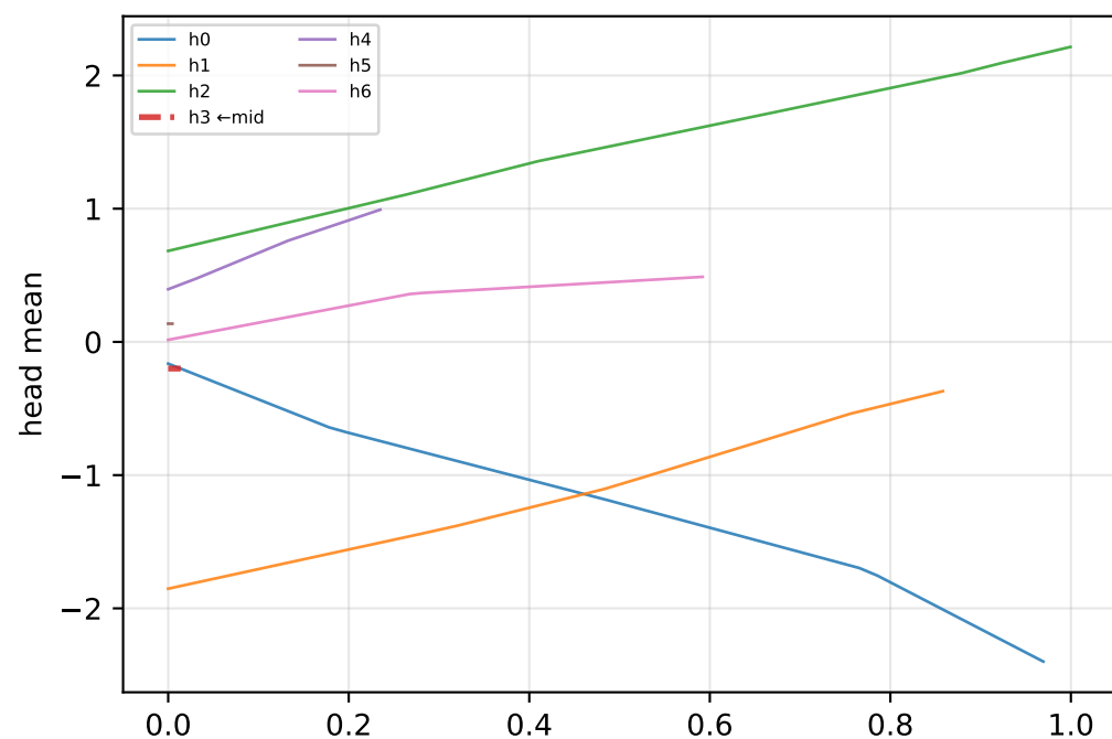
piecewise k=7 | mid_idx=3
