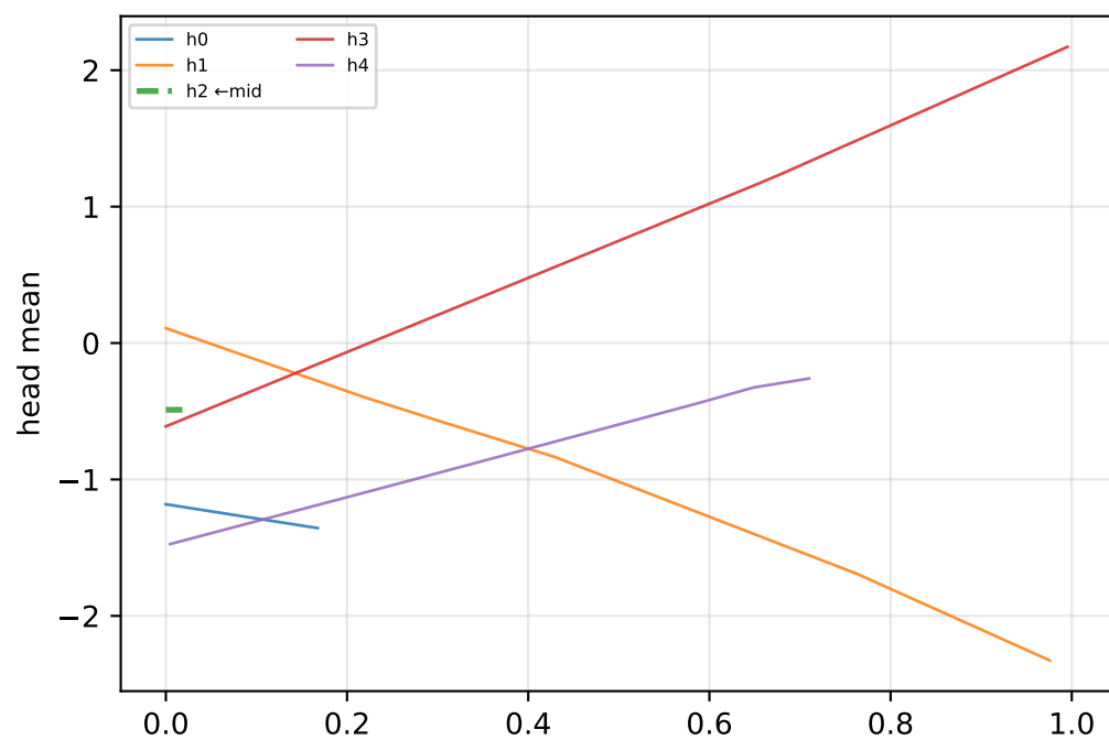
piecewise k=5 | mid_idx=2
