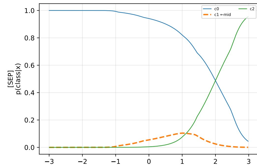
exponential k=3 | mid_idx=1
