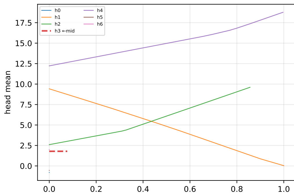
exponential k=7 | mid_idx=3
