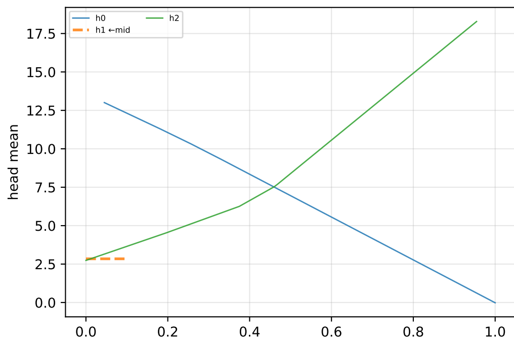
exponential k=3 | mid_idx=1
