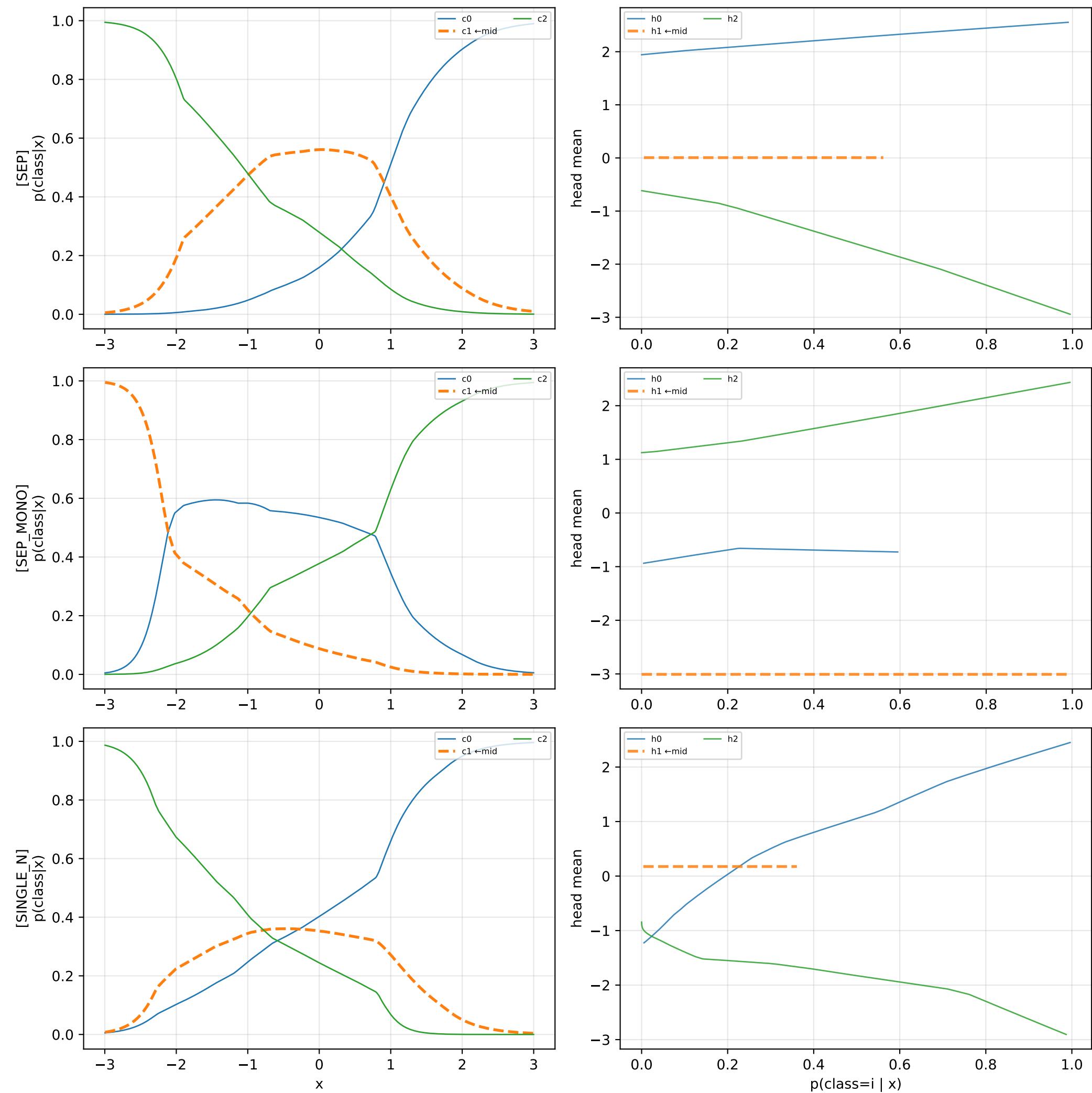
bimodal k=3 | mid_idx=1
