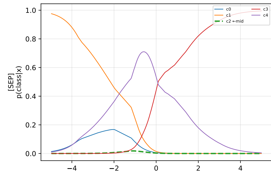
piecewise k=5 | mid_idx=2
