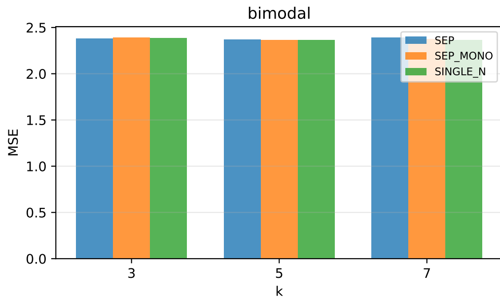
MSE by variant — D1 (strategy) and D3 (monotonic constraints)
