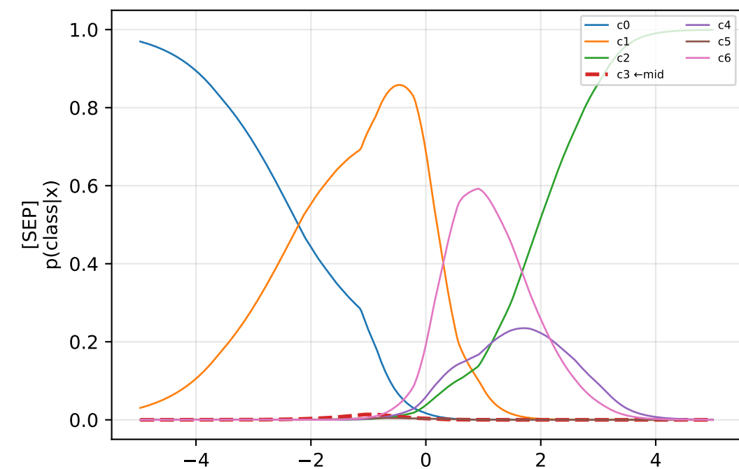
piecewise k=7 | mid_idx=3
