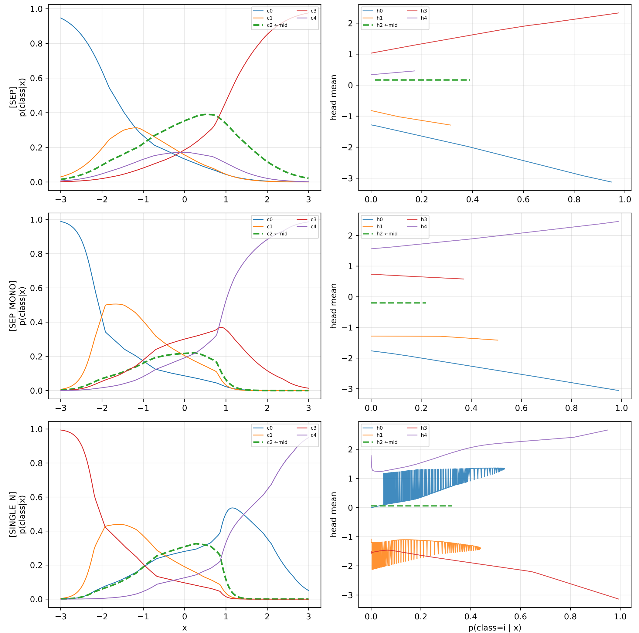
bimodal k=5 | mid_idx=2
