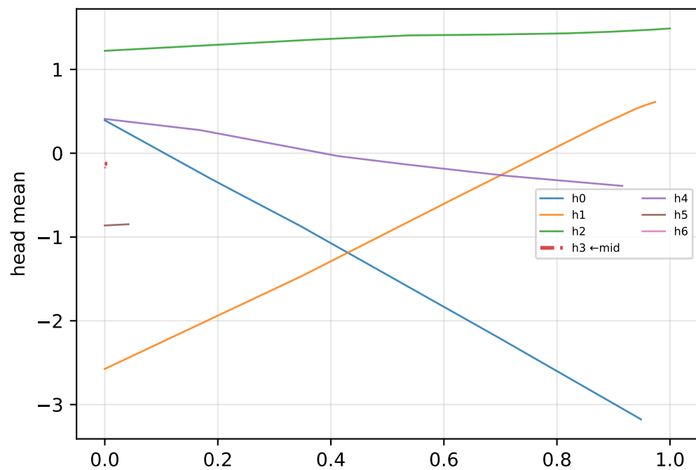
heteroscedastic k=7 | mid_idx=3
