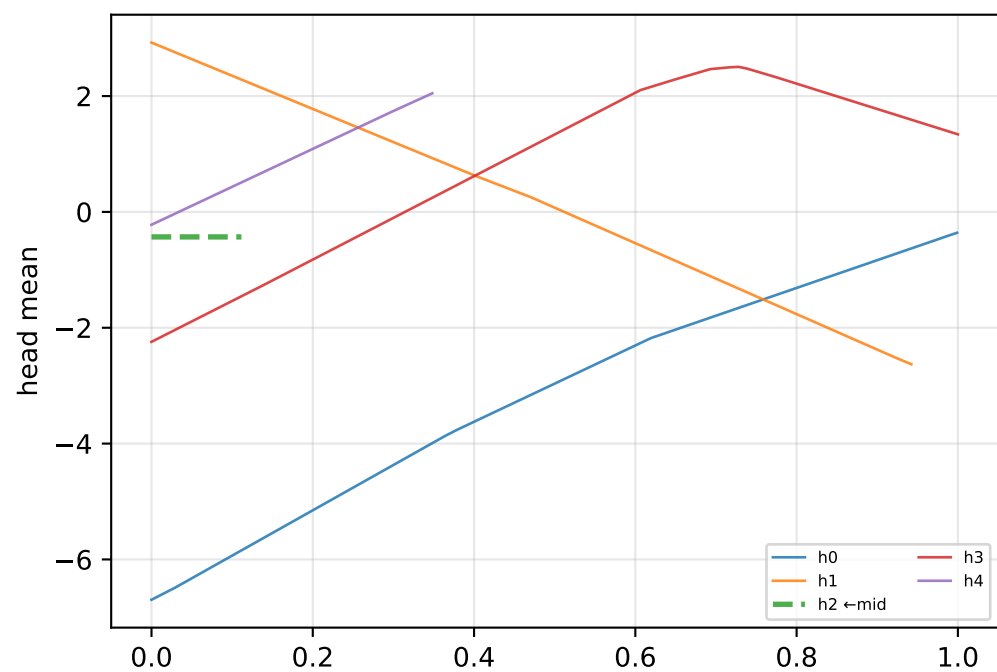
heteroscedastic k=5 | mid_idx=2
