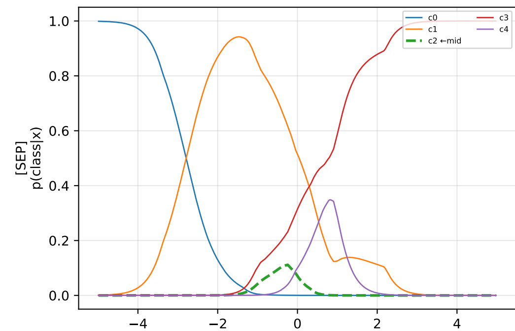
heteroscedastic k=5 | mid_idx=2
