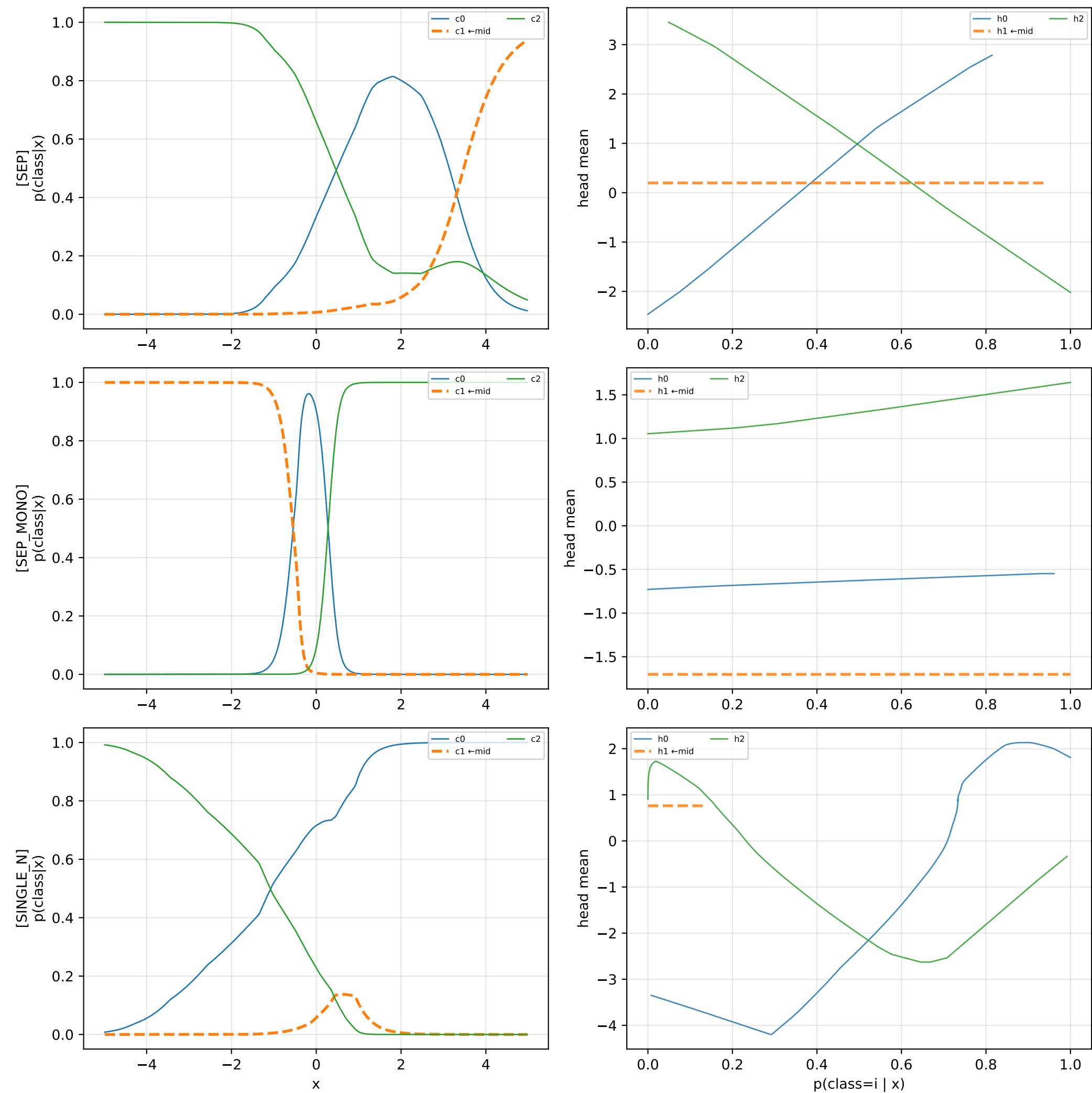
heteroscedastic k=3 | mid_idx=1
