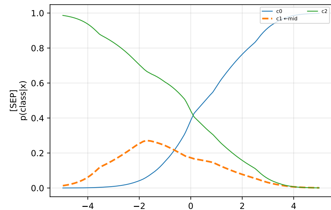
piecewise k=3 | mid_idx=1
