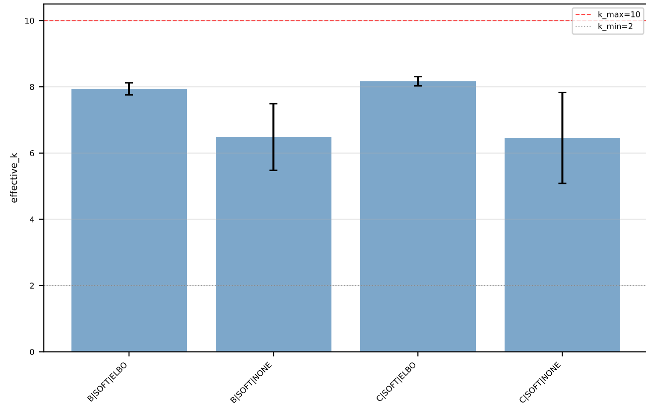
piecewise k_max=10 — effective_k by config
