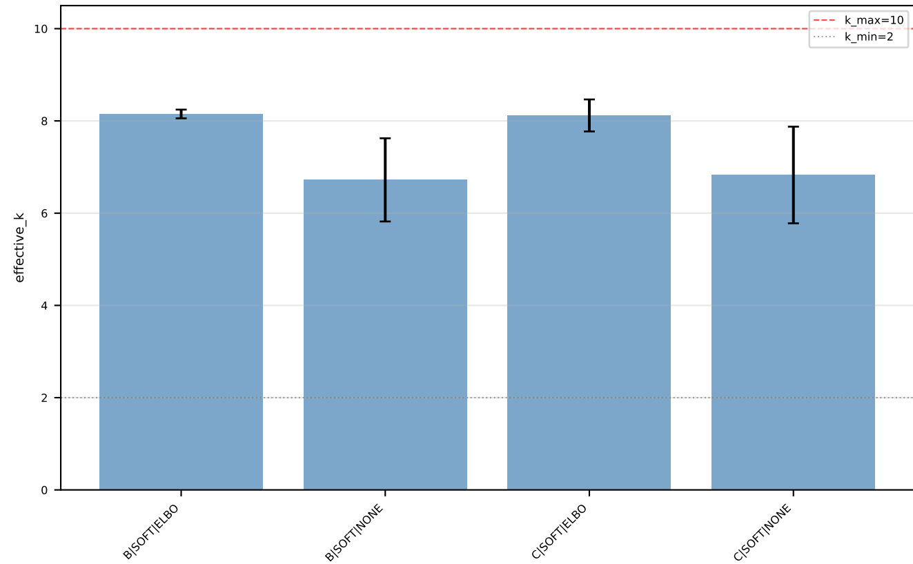
heteroscedastic k_max=10 — effective_k by config
