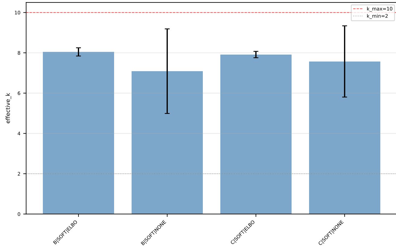
exponential k_max=10 — effective_k by config
