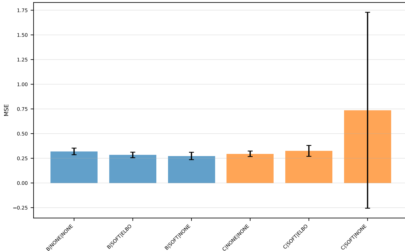
piecewise k_max=10 — MSE (B=blue, C=orange)
