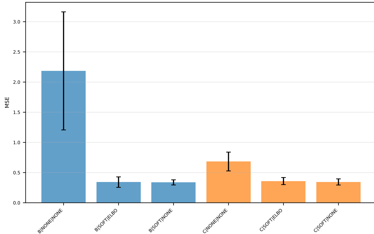
exponential k_max=10 — MSE (B=blue, C=orange)
