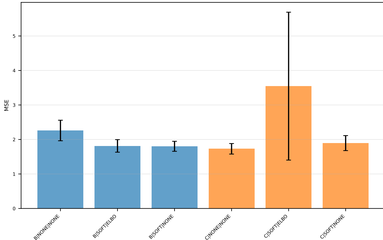
heteroscedastic k_max=10 — MSE (B=blue, C=orange)
