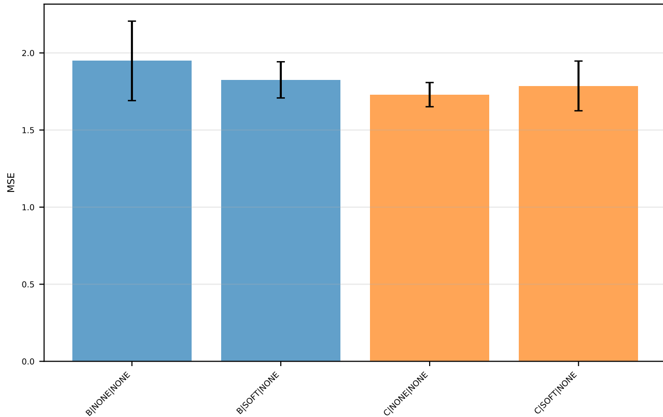
heteroscedastic k_max=20 — MSE (B=blue, C=orange)
