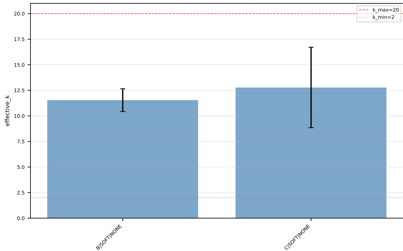
piecewise k_max=20 — effective_k by config
