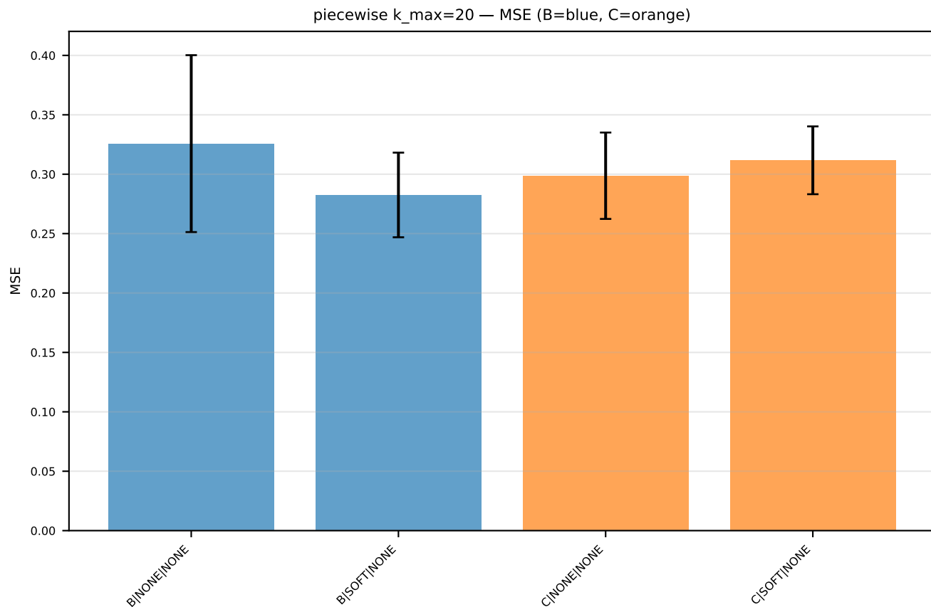
piecewise k_max=20
