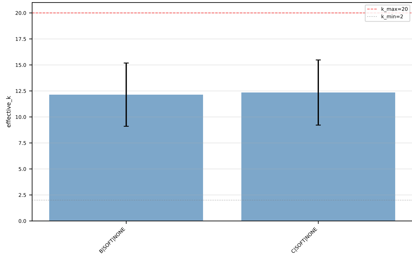
heteroscedastic k_max=20 — effective_k by config
