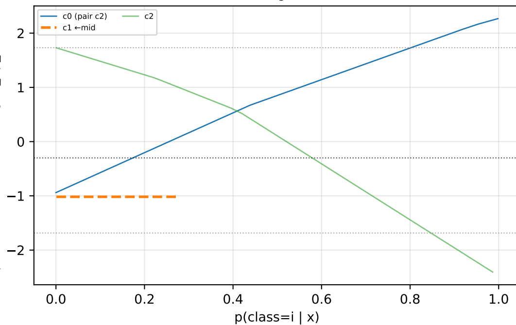
[ProbReg] k=3
