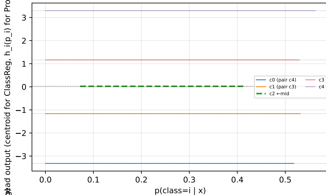
[ProbReg] k=5
