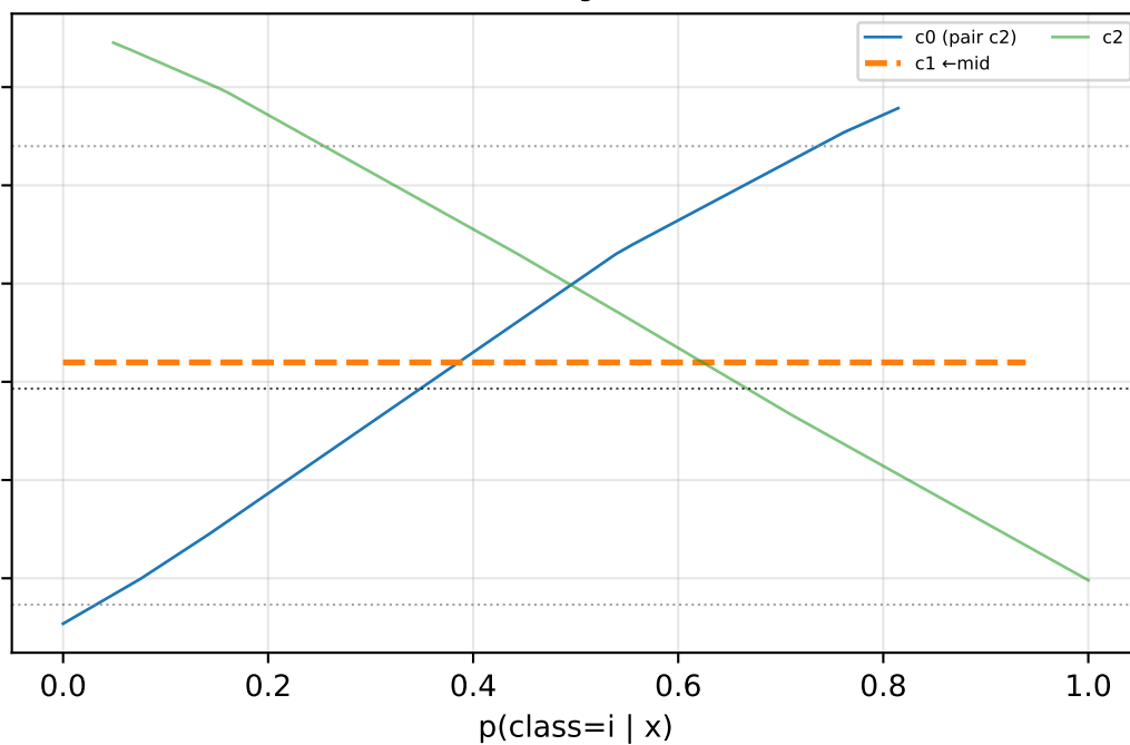
[ProbReg] k=3
