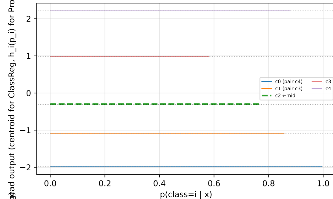
[ProbReg] k=5
