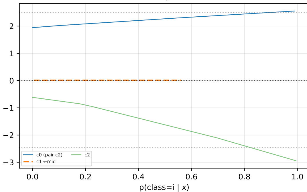
[ProbReg] k=3
