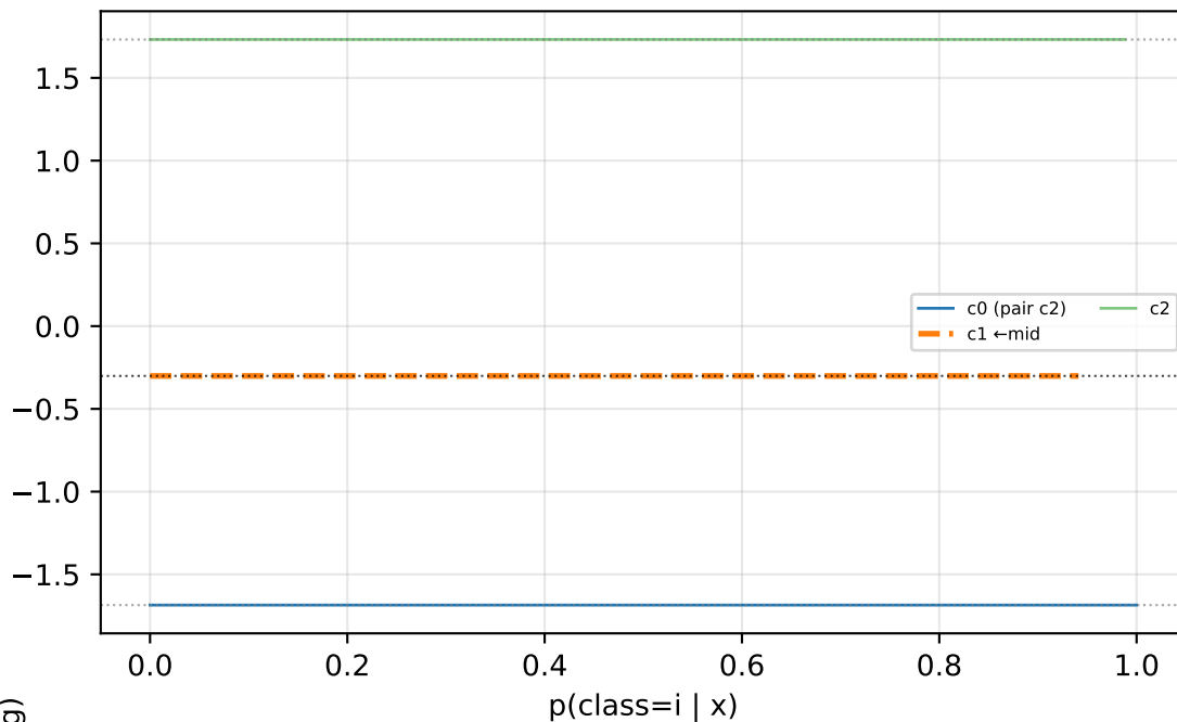
[ProbReg] k=3
