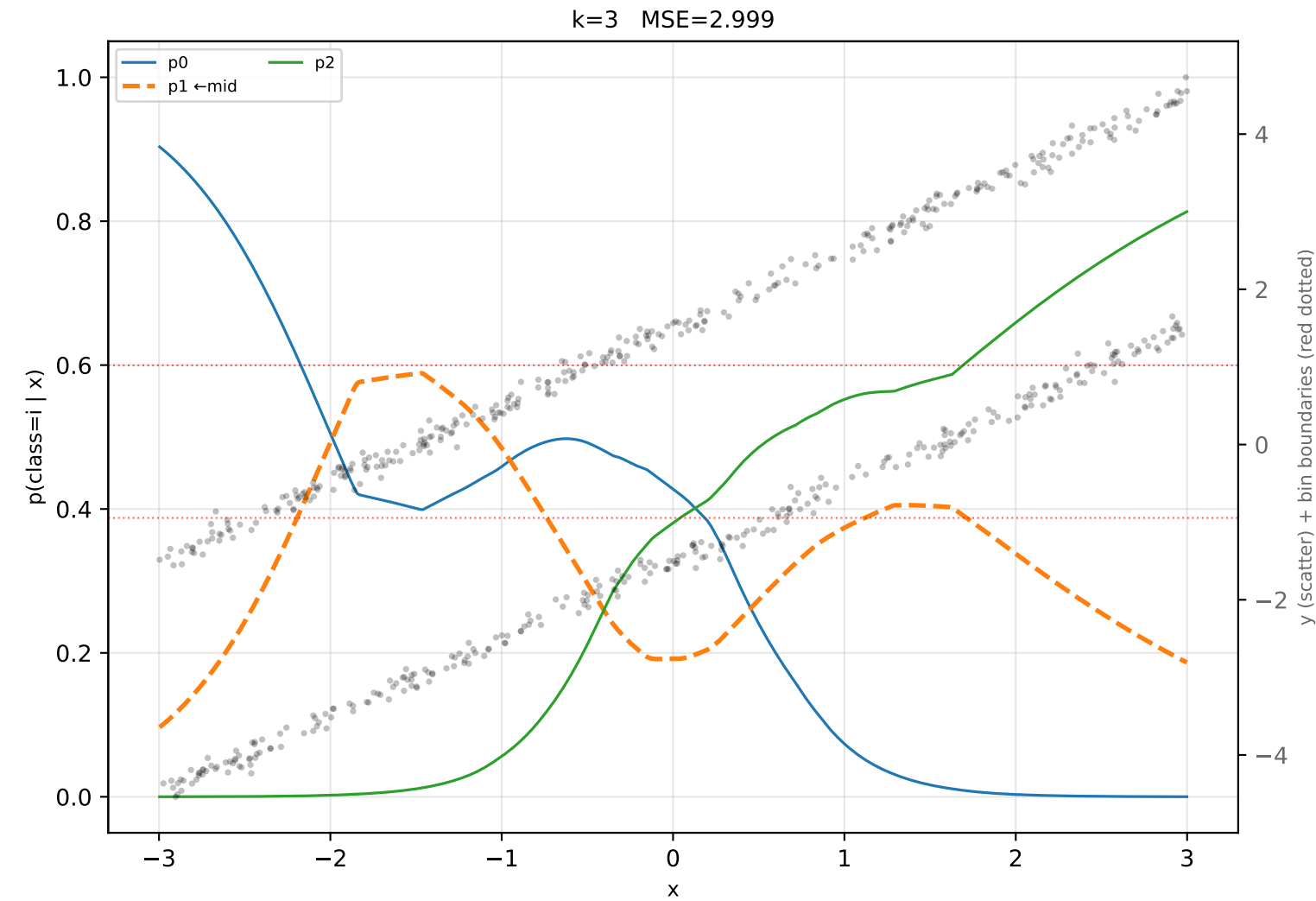
bimodal — ClassReg classifier probabilities p_i(x)
