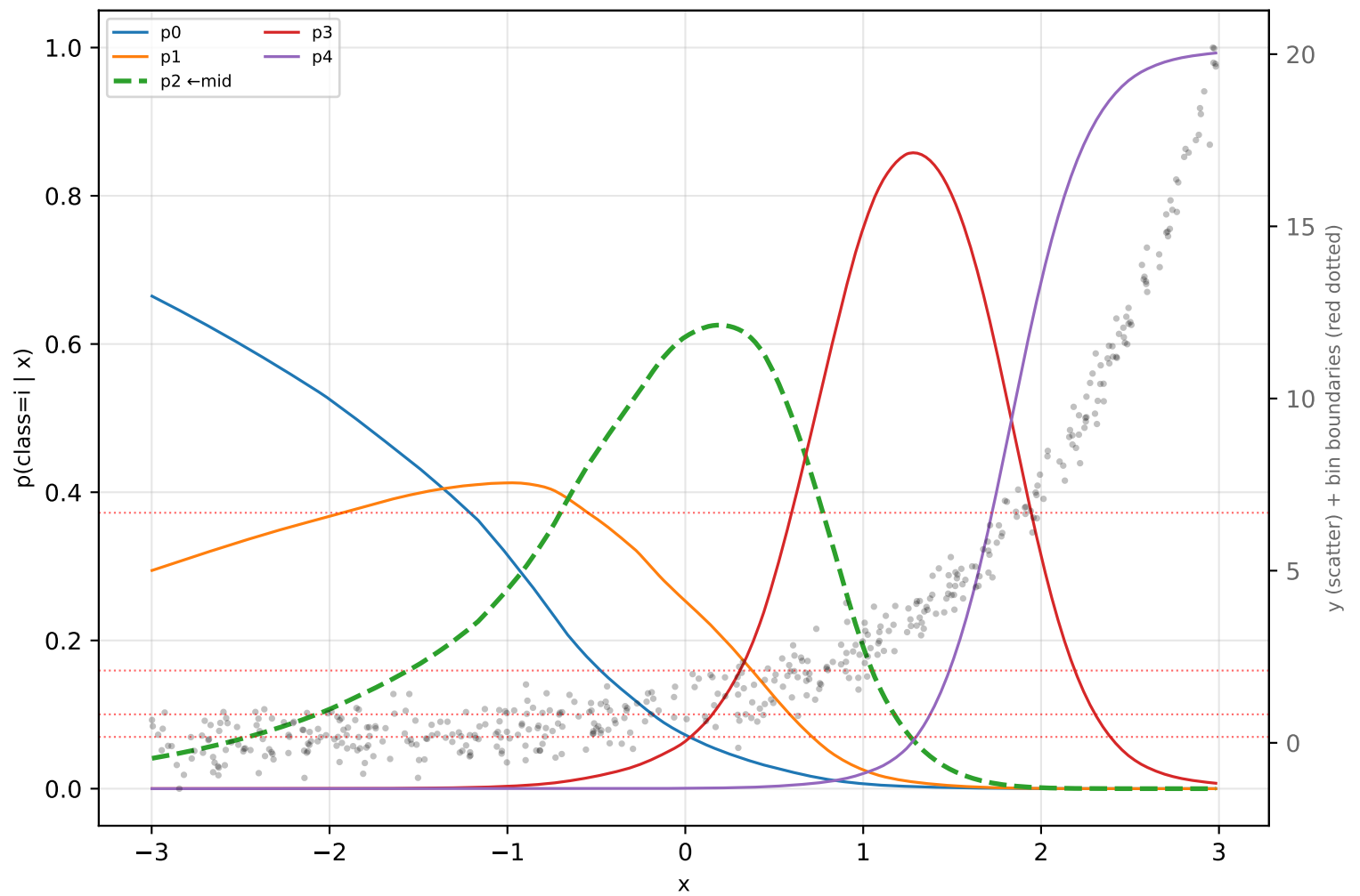
exponential — ClassReg classifier probabilities p_i(x)
