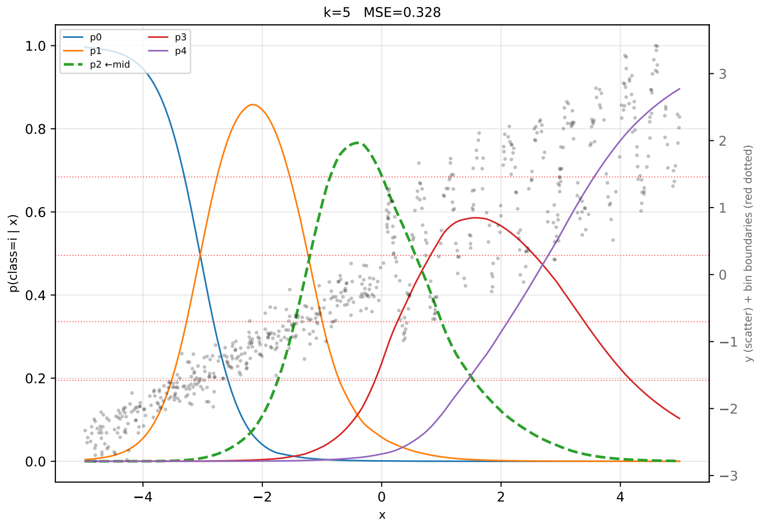
piecewise — ClassReg classifier probabilities p_i(x)
