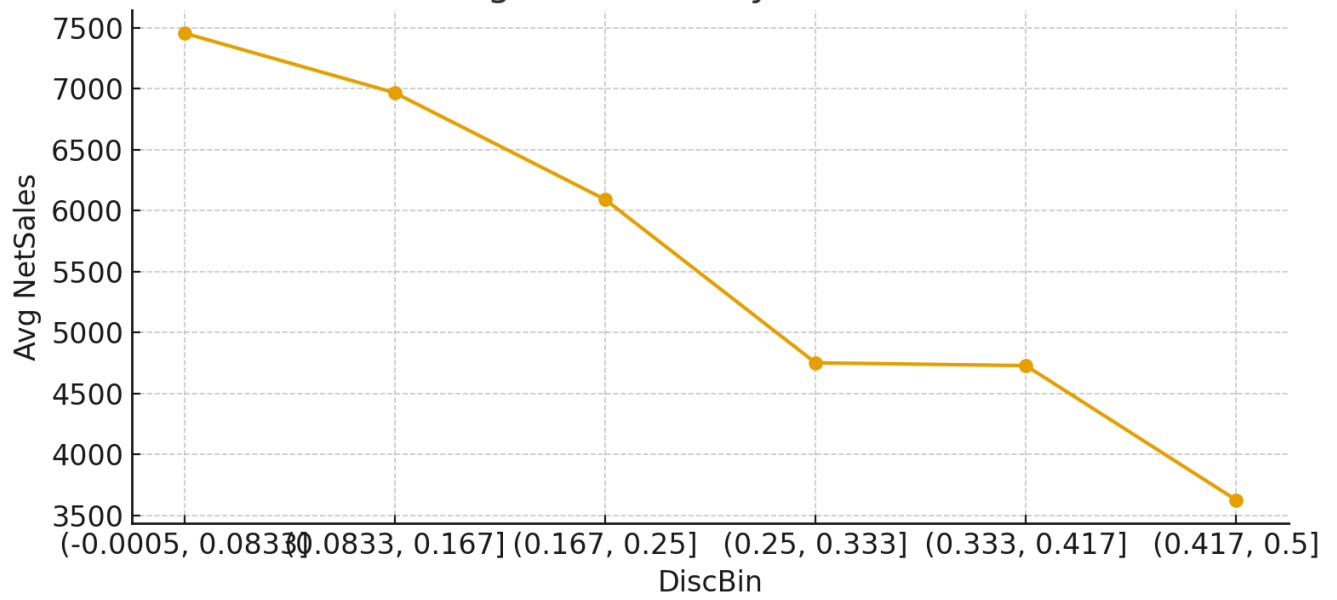
Average NetSales by Discount Bins
