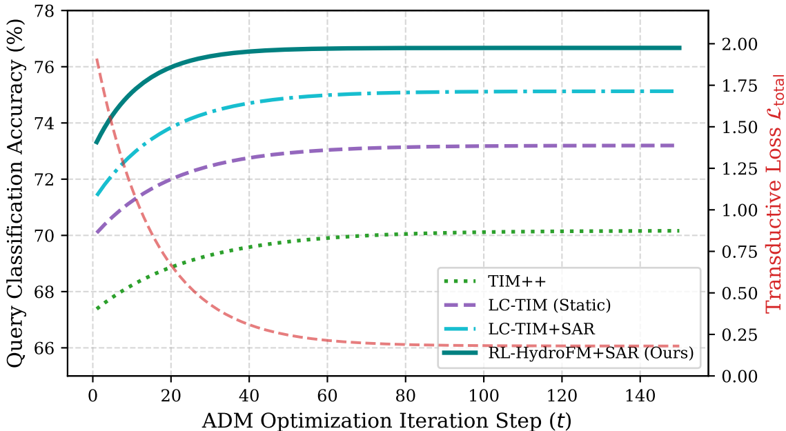
ADM Transductive Optimization Convergence Trajectory
