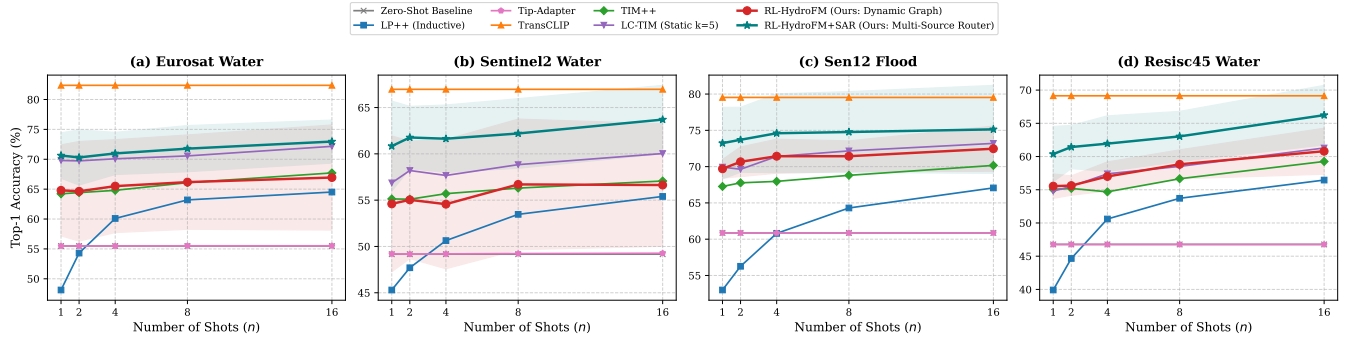
Fig. 1: Few-shot classification performance comparison (Top-1 Accuracy % vs. Number of Shots n \in \{1, 2, 4, 8, 16\} ) across four Earth observation water resources benchmarks: (a) EuroSAT-Water, (b) Sentinel-2 Water Bodies, (c) Sen12-Flood, and (d) RESISC45-Water. Curves and error bands denote mean and standard deviation over 5 independent random seeds. RL-HYDROFM+SAR (teal star) and RL-HYDROFM (red circle) consistently achieve superior accuracy across all shot regimes, with the most pronounced gains in the extreme low-shot regime (1-shot and 2-shot).
