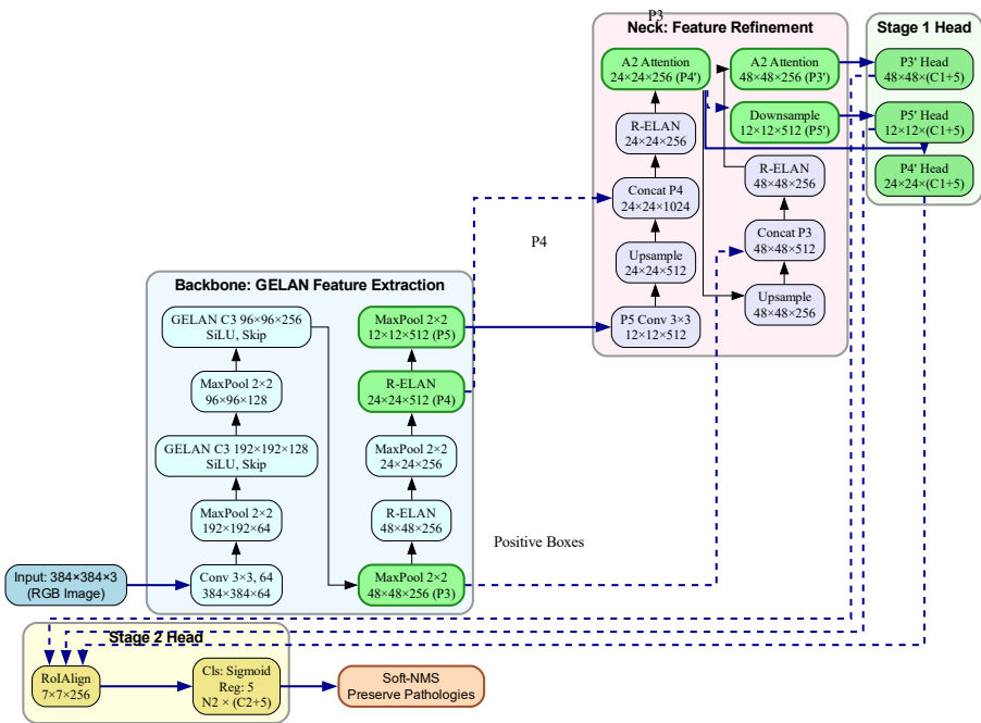
YOLOspine: A Two-Stage Attention-Enhanced Framework for Multi-Label Detection of Lumbar Spinal Pathologies in MRI
