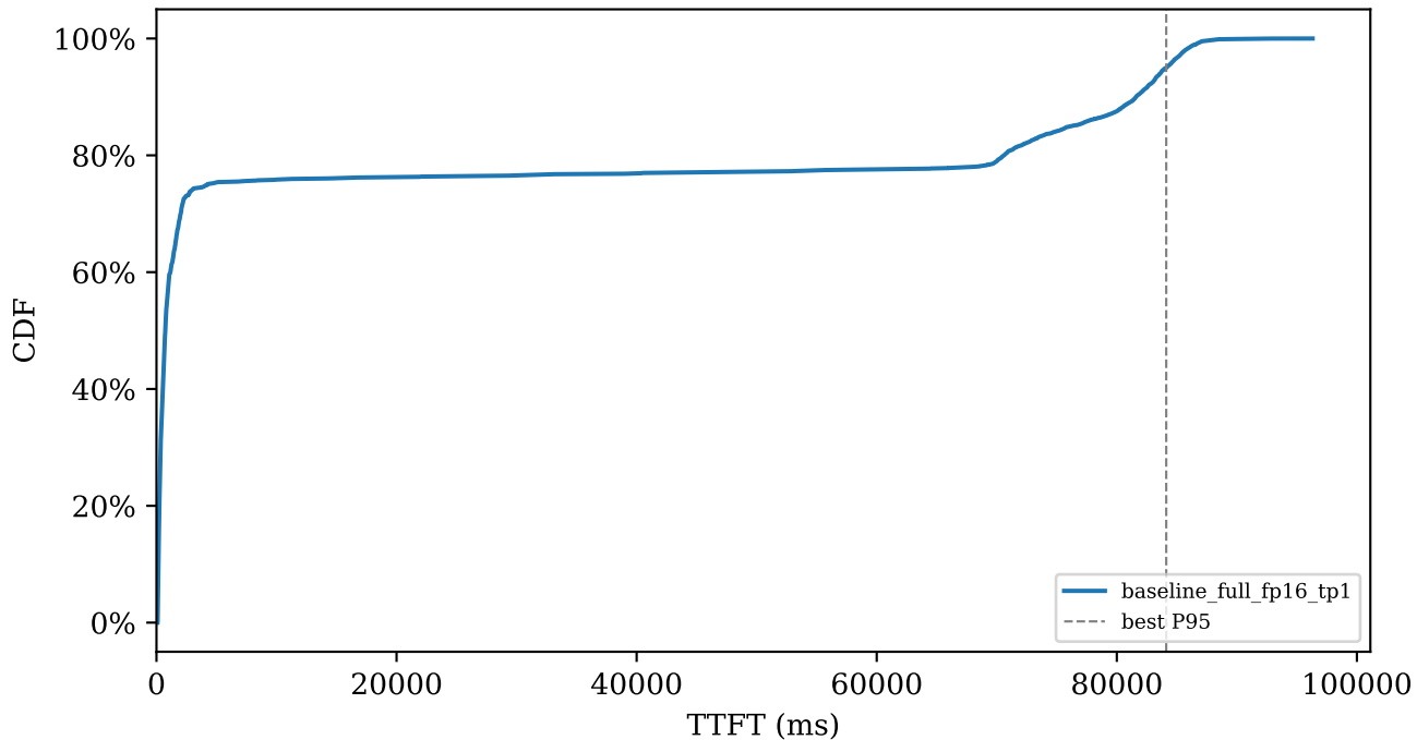
TTFT CDF by Execution Strategy
