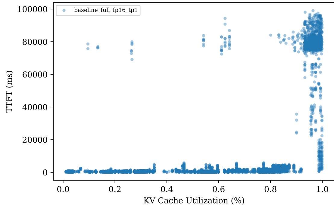
KV Cache Pressure vs. TTFT
